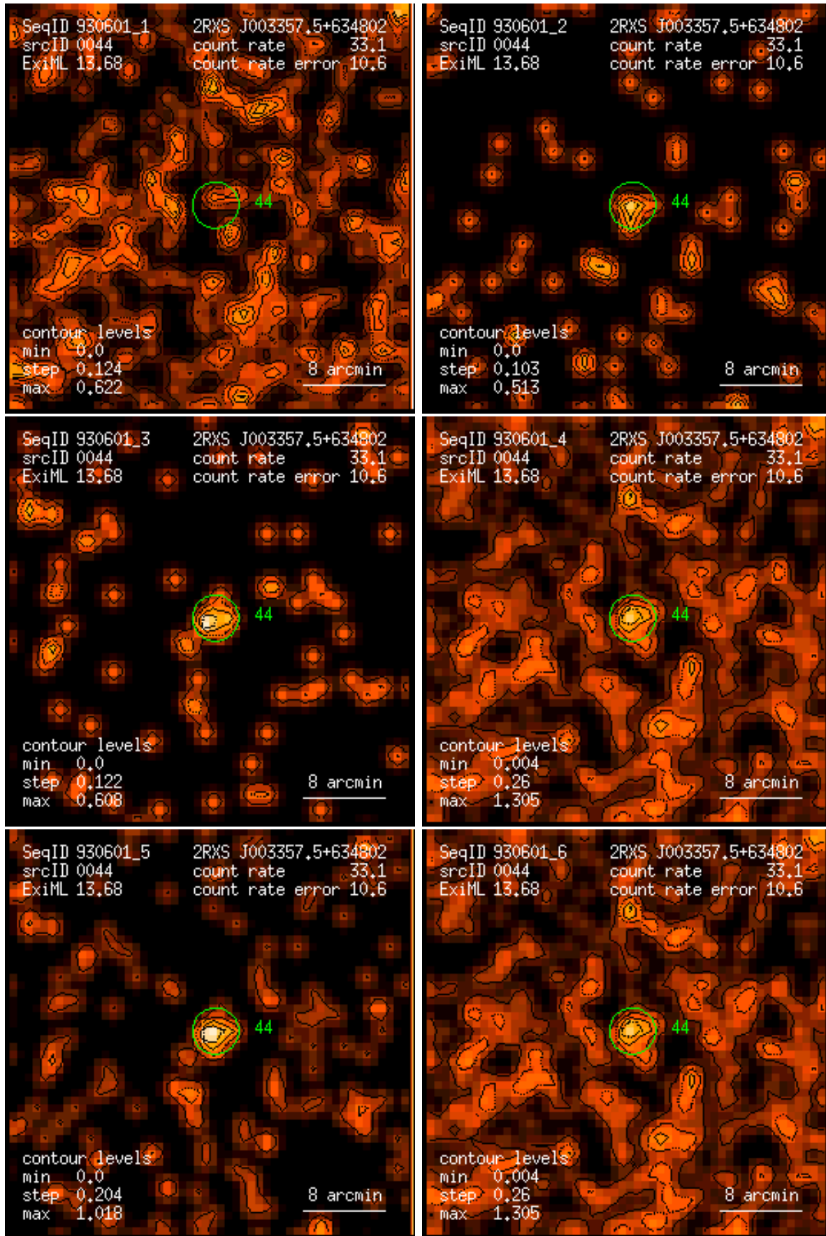
Figure 44: RASS 930601: detection 0044: band rate images, Gaussian filter: (1) PSPC channels 11 – 41, (2) 52 – 90, (3) 91 – 201, (4) 11 – 235, (5) 52 – 201, (6) 11 – 201. Broad band rates in counts/ks. Band rate contour levels in counts/ks/arcmin 2 .
