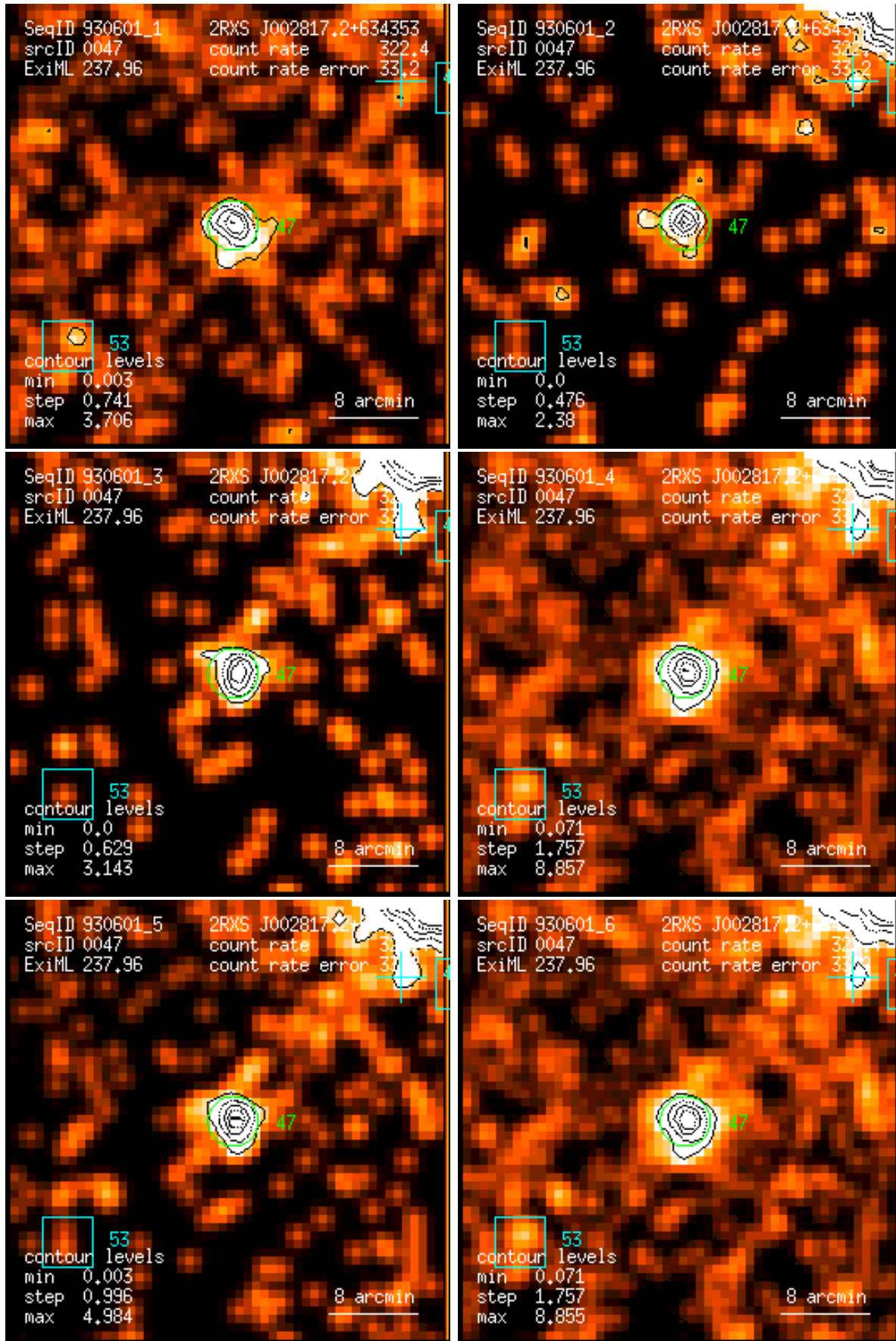
Figure 47: RASS 930601: detection 0047: band rate images, Gaussian filter: (1) PSPC channels 11 – 41, (2) 52 – 90, (3) 91 – 201, (4) 11 – 235, (5) 52 – 201, (6) 11 – 201. Broad band rates in counts/ks. Band rate contour levels in counts/ks/arcmin 2 .
