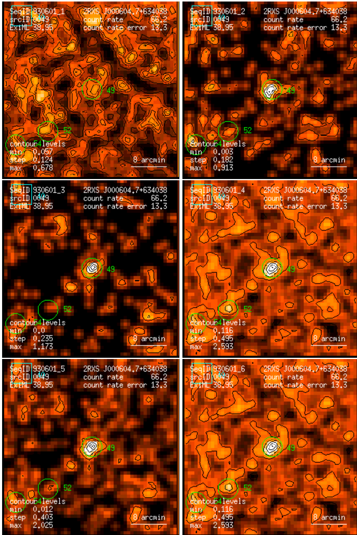
Figure 49: RASS 930601: detection 0049: band rate images, Gaussian filter: (1) PSPC channels 11 – 41, (2) 52 – 90, (3) 91 – 201, (4) 11 – 235, (5) 52 – 201, (6) 11 – 201. Broad band rates in counts/ks. Band rate contour levels in counts/ks/arcmin 2 .
