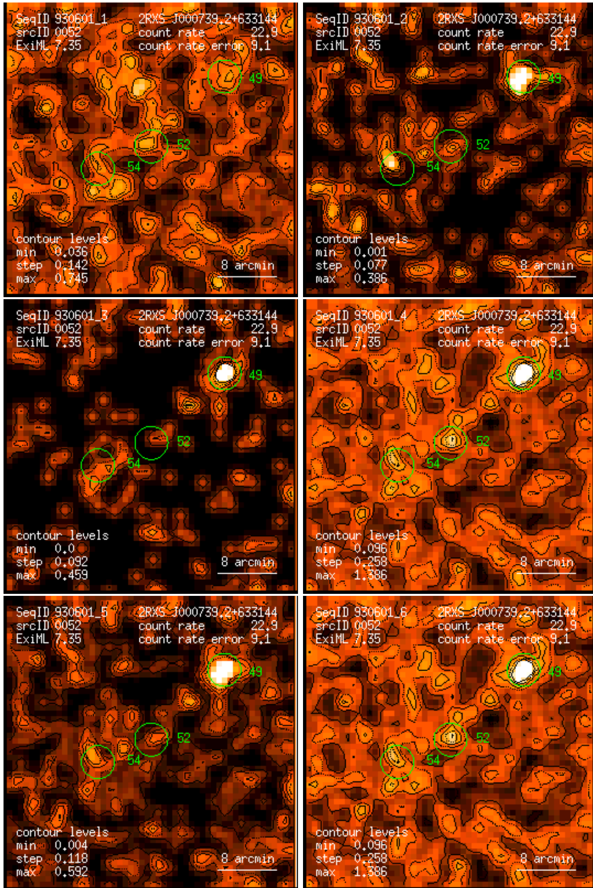
Figure 52: RASS 930601: detection 0052: band rate images, Gaussian filter: (1) PSPC channels 11 – 41, (2) 52 – 90, (3) 91 – 201, (4) 11 – 235, (5) 52 – 201, (6) 11 – 201. Broad band rates in counts/ks. Band rate contour levels in counts/ks/arcmin 2 .
