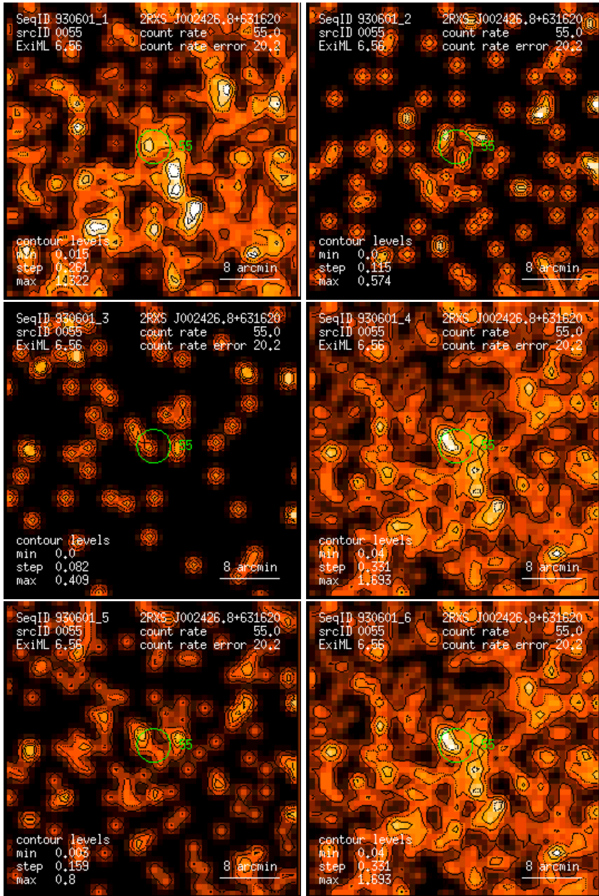
Figure 55: RASS 930601: detection 0055: band rate images, Gaussian filter: (1) PSPC channels 11 – 41, (2) 52 – 90, (3) 91 – 201, (4) 11 – 235, (5) 52 – 201, (6) 11 – 201. Broad band rates in counts/ks. Band rate contour levels in counts/ks/arcmin 2 .
