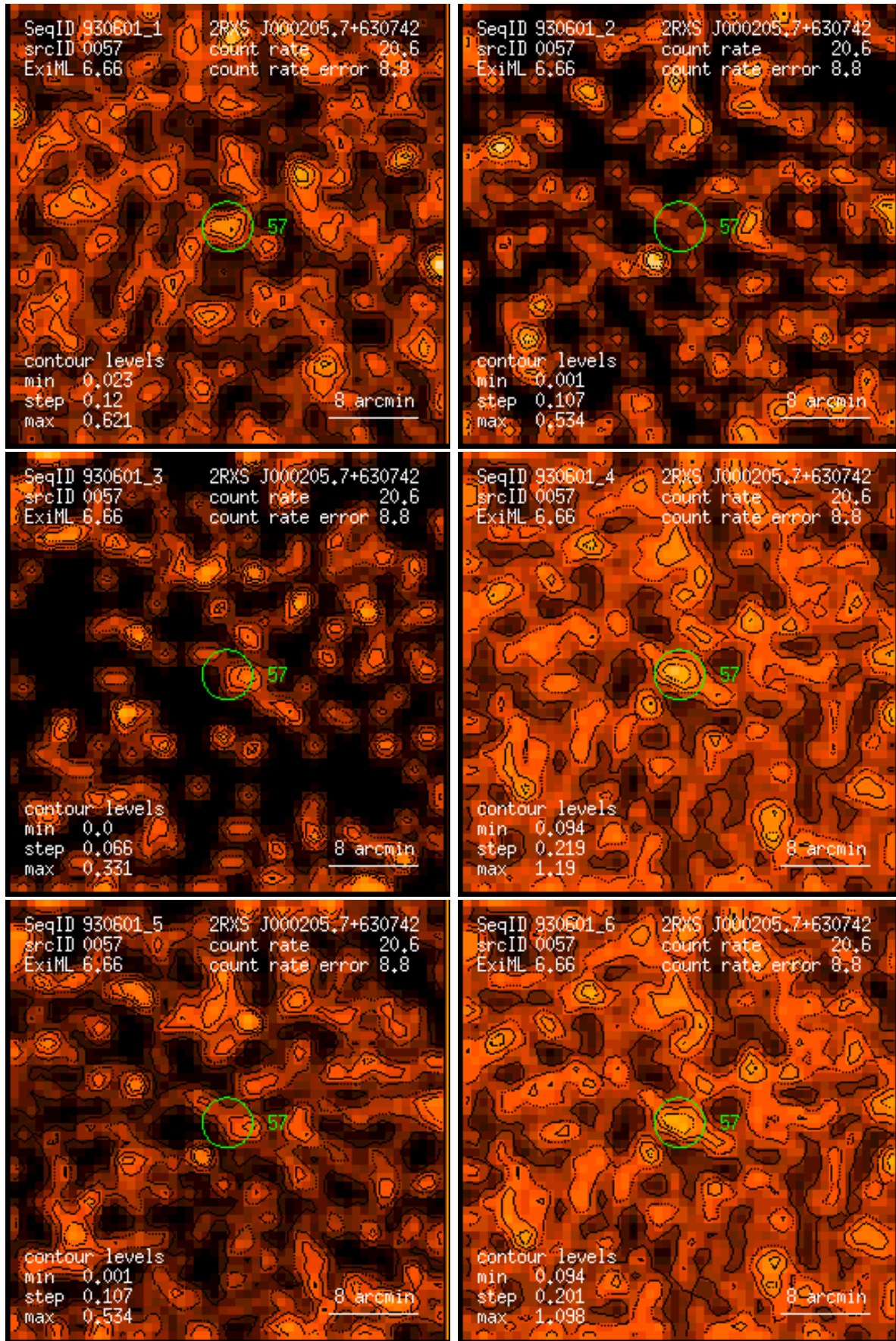
Figure 57: RASS 930601: detection 0057: band rate images, Gaussian filter: (1) PSPC channels 11 – 41, (2) 52 – 90, (3) 91 – 201, (4) 11 – 235, (5) 52 – 201, (6) 11 – 201. Broad band rates in counts/ks. Band rate contour levels in counts/ks/arcmin 2 .
