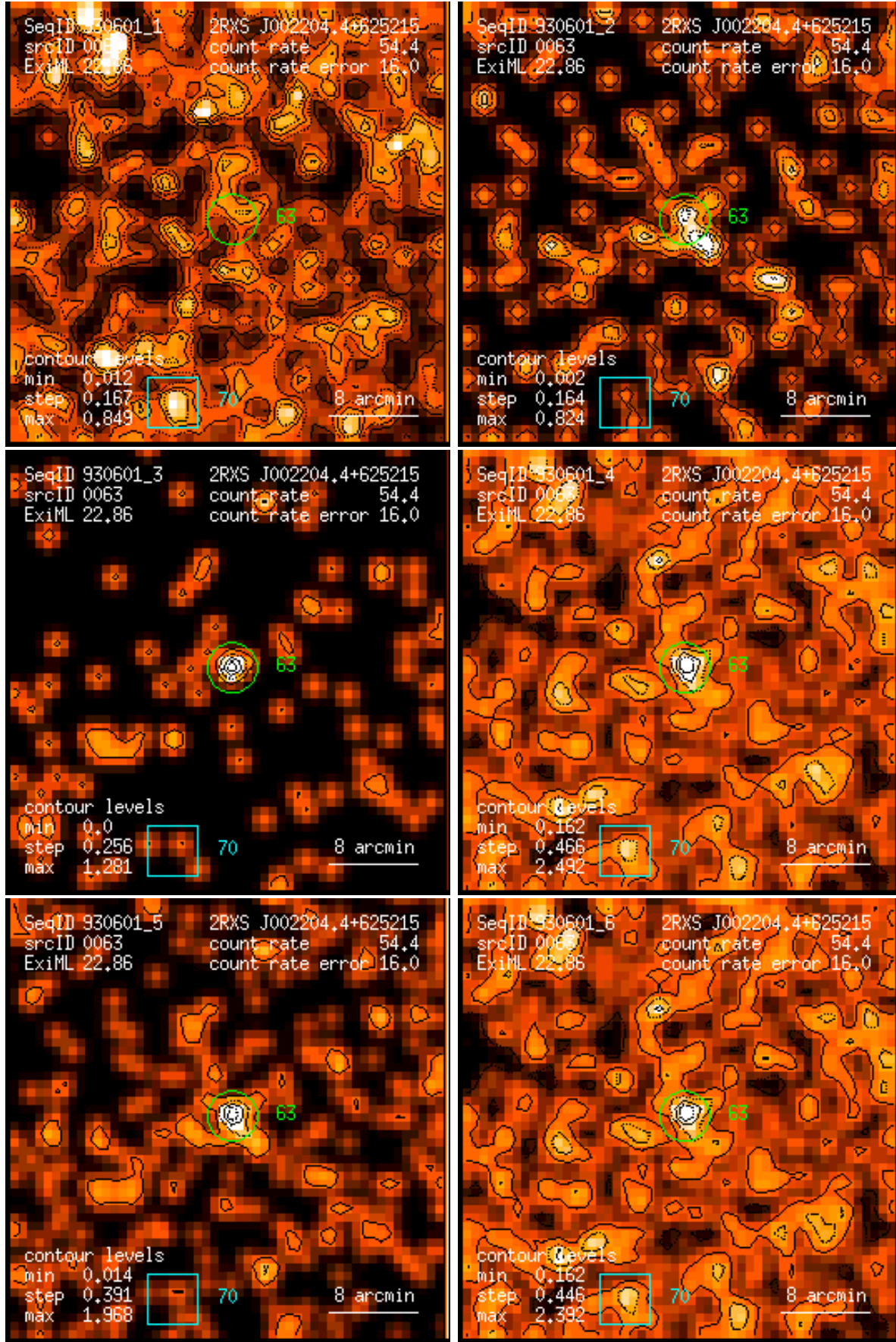
Figure 63: RASS 930601: detection 0063: band rate images, Gaussian filter: (1) PSPC channels 11 – 41, (2) 52 – 90, (3) 91 – 201, (4) 11 – 235, (5) 52 – 201, (6) 11 – 201. Broad band rates in counts/ks. Band rate contour levels in counts/ks/arcmin 2 .
