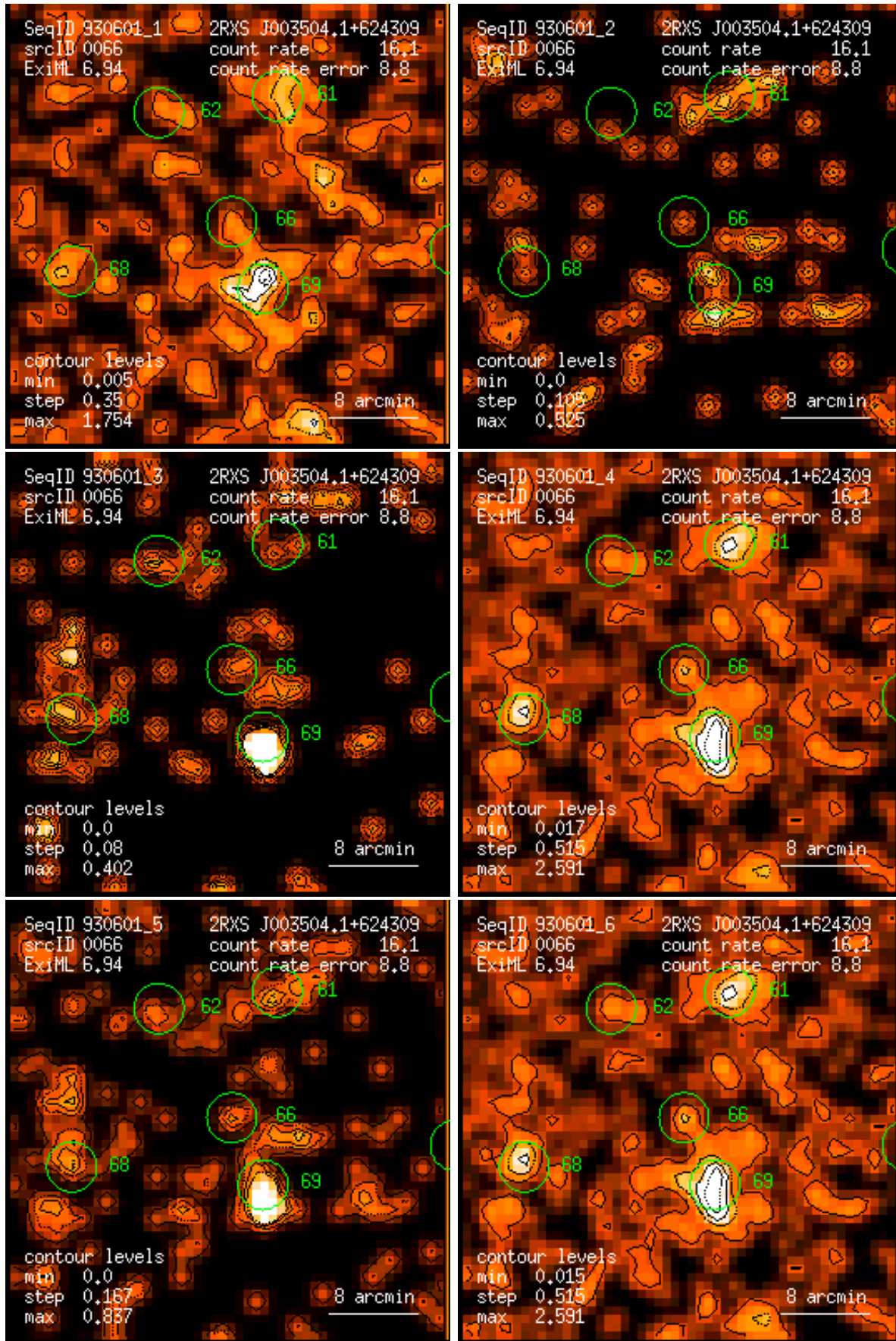
Figure 66: RASS 930601: detection 0066: band rate images, Gaussian filter: (1) PSPC channels 11 – 41, (2) 52 – 90, (3) 91 – 201, (4) 11 – 235, (5) 52 – 201, (6) 11 – 201. Broad band rates in counts/ks. Band rate contour levels in counts/ks/arcmin 2 .
