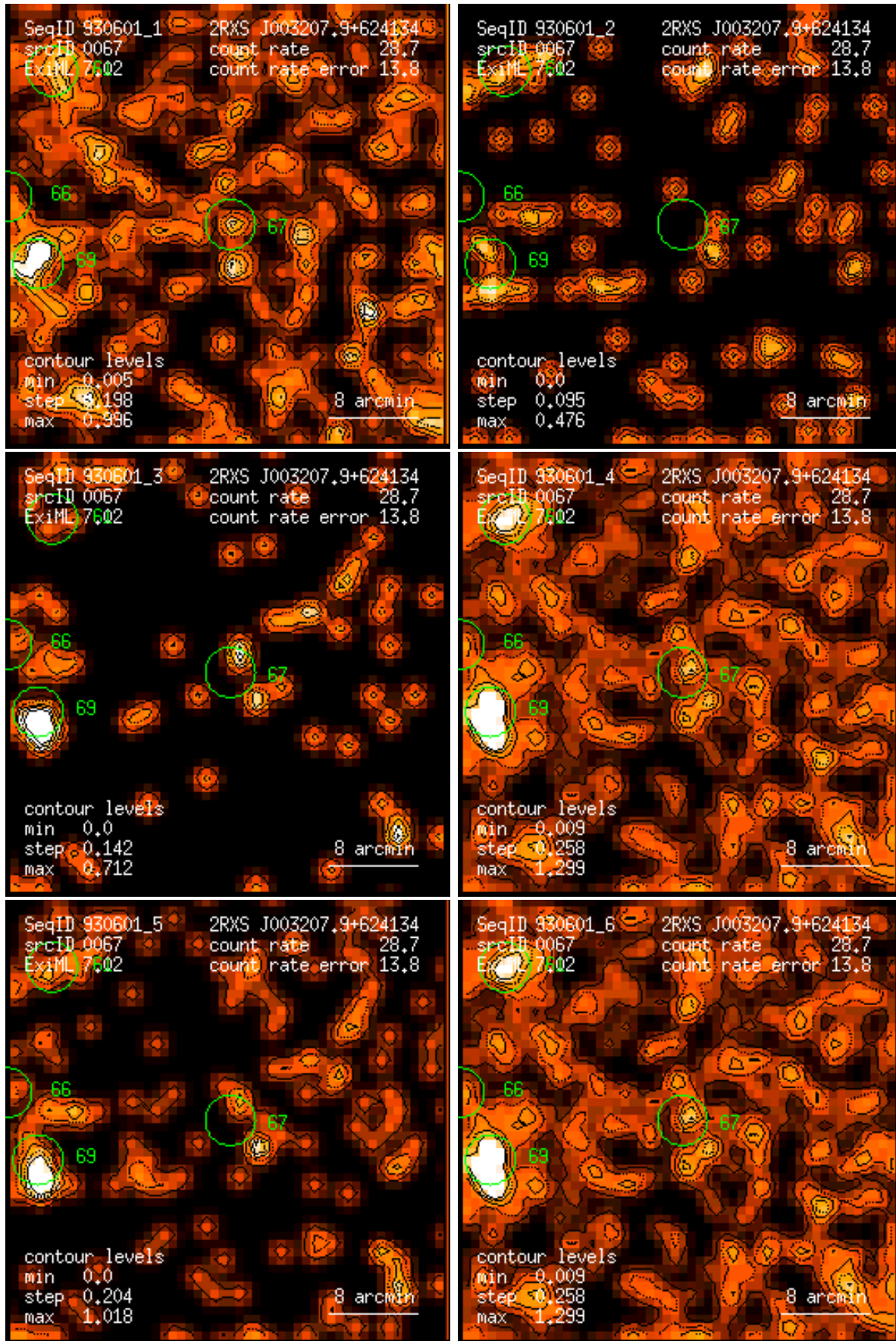
Figure 67: RASS 930601: detection 0067: band rate images, Gaussian filter: (1) PSPC channels 11 – 41, (2) 52 – 90, (3) 91 – 201, (4) 11 – 235, (5) 52 – 201, (6) 11 – 201. Broad band rates in counts/ks. Band rate contour levels in counts/ks/arcmin 2 .
