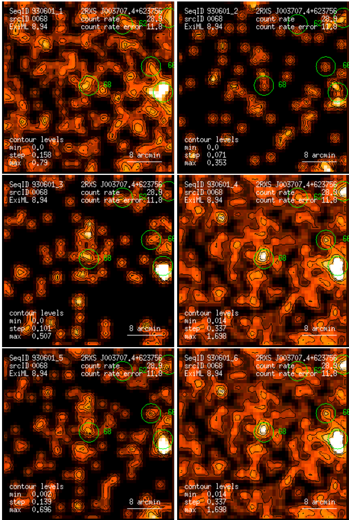
Figure 68: RASS 930601: detection 0068: band rate images, Gaussian filter: (1) PSPC channels 11 – 41, (2) 52 – 90, (3) 91 – 201, (4) 11 – 235, (5) 52 – 201, (6) 11 – 201. Broad band rates in counts/ks. Band rate contour levels in counts/ks/arcmin 2 .
