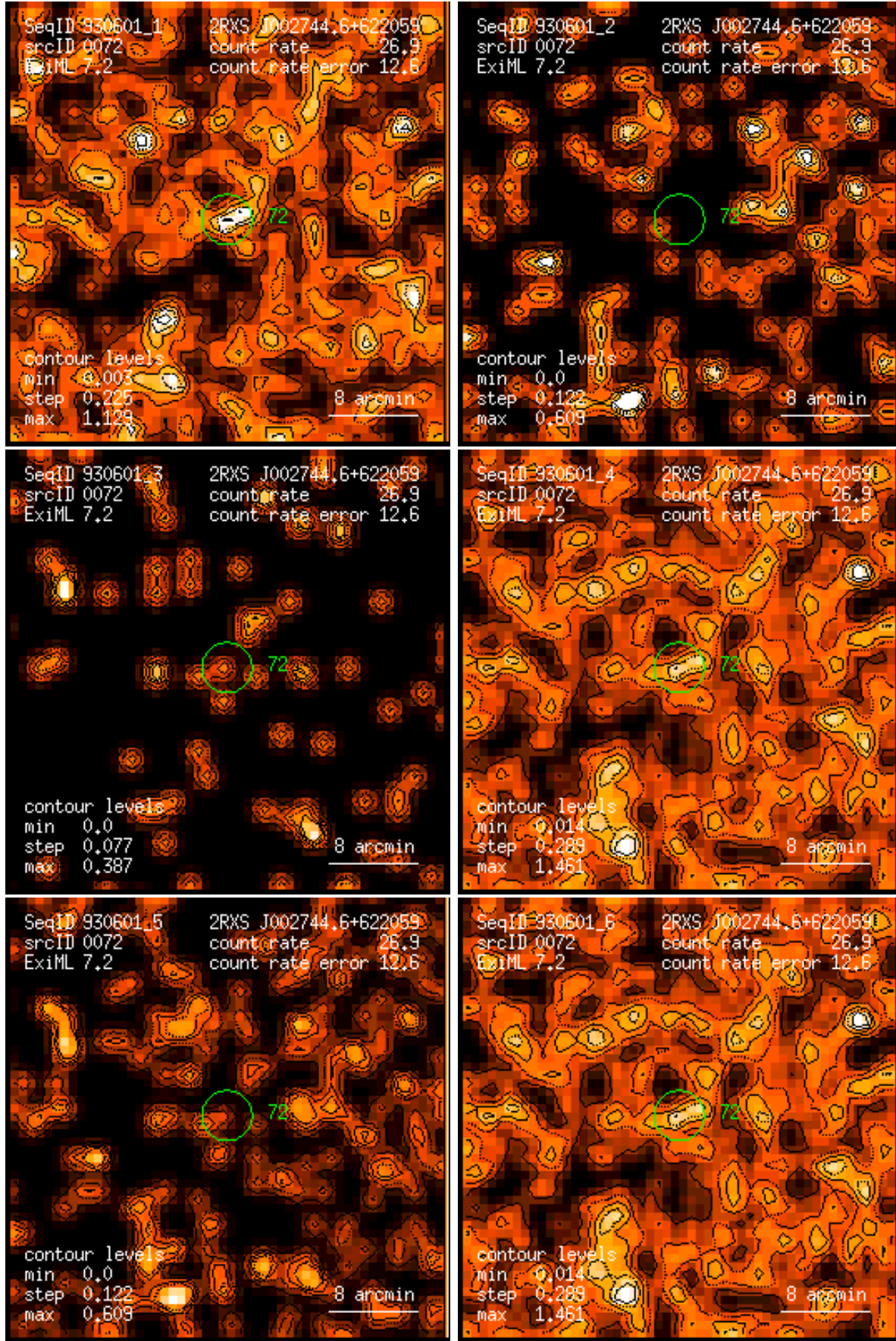
Figure 72: RASS 930601: detection 0072: band rate images, Gaussian filter: (1) PSPC channels 11 – 41, (2) 52 – 90, (3) 91 – 201, (4) 11 – 235, (5) 52 – 201, (6) 11 – 201. Broad band rates in counts/ks. Band rate contour levels in counts/ks/arcmin 2 .
