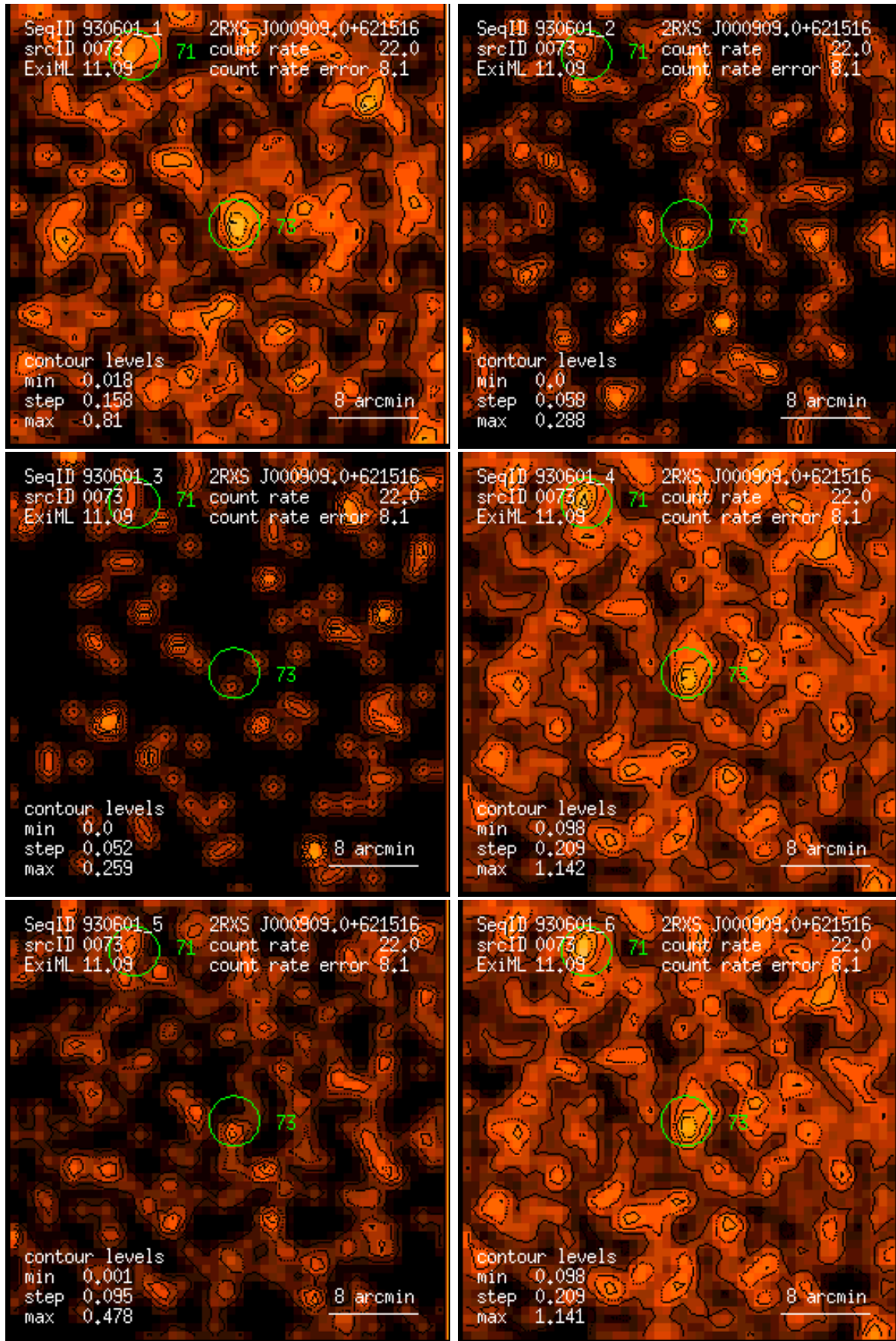
Figure 73: RASS 930601: detection 0073: band rate images, Gaussian filter: (1) PSPC channels 11 – 41, (2) 52 – 90, (3) 91 – 201, (4) 11 – 235, (5) 52 – 201, (6) 11 – 201. Broad band rates in counts/ks. Band rate contour levels in counts/ks/arcmin 2 .
