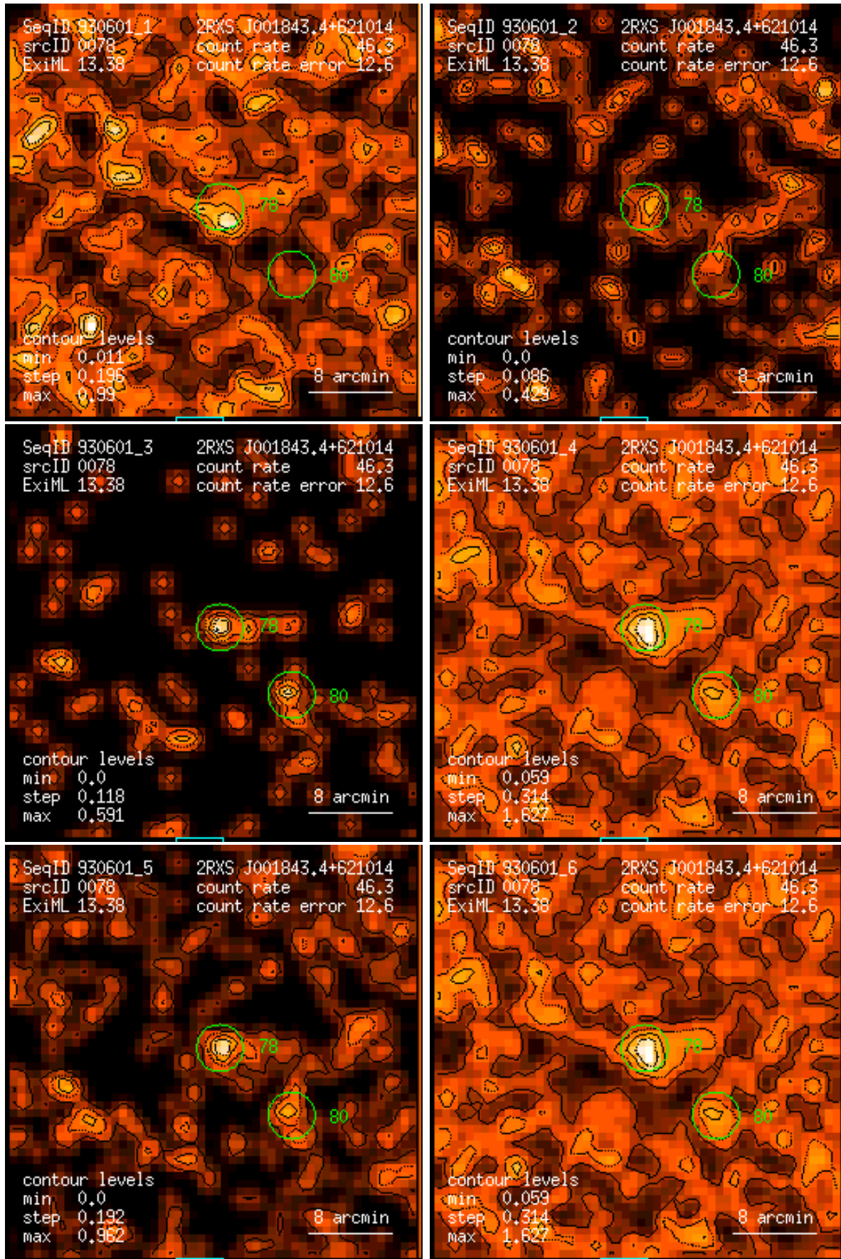
Figure 78: RASS 930601: detection 0078: band rate images, Gaussian filter: (1) PSPC channels 11 – 41, (2) 52 – 90, (3) 91 – 201, (4) 11 – 235, (5) 52 – 201, (6) 11 – 201. Broad band rates in counts/ks. Band rate contour levels in counts/ks/arcmin 2 .
