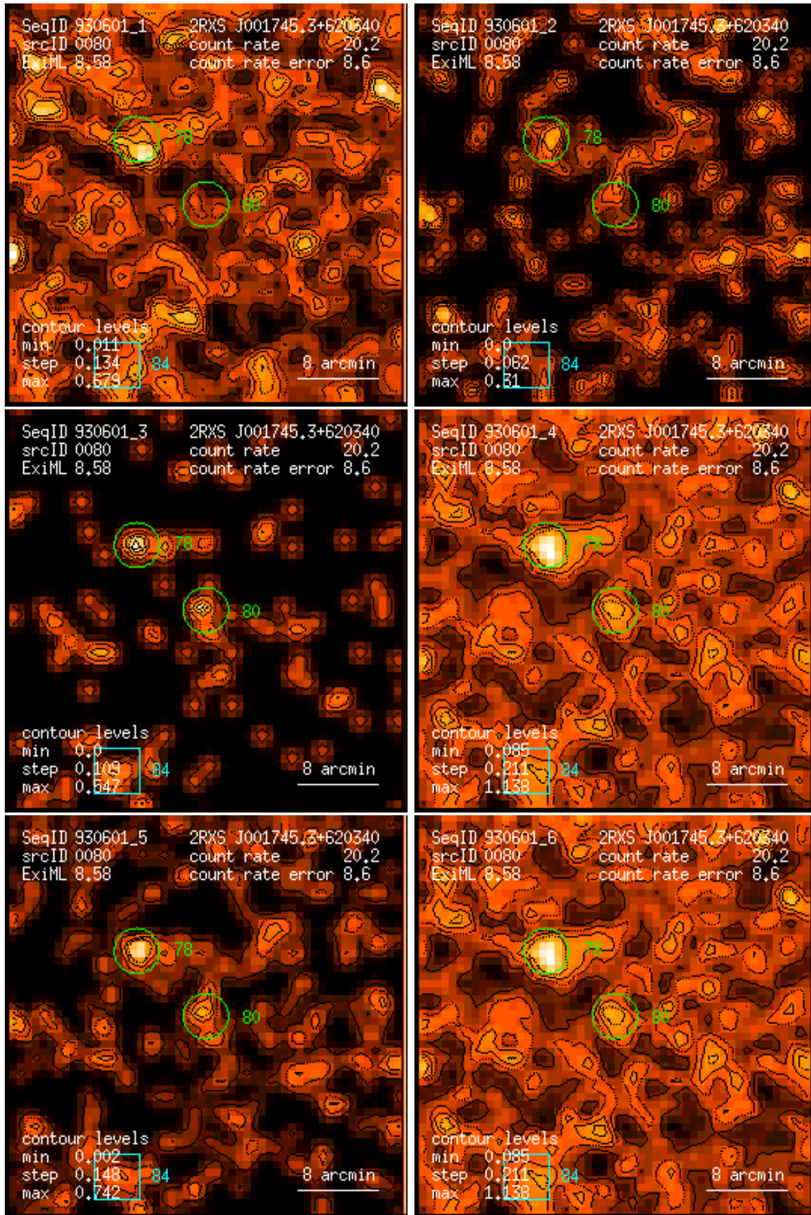
Figure 80: RASS 930601: detection 0080: band rate images, Gaussian filter: (1) PSPC channels 11 – 41, (2) 52 – 90, (3) 91 – 201, (4) 11 – 235, (5) 52 – 201, (6) 11 – 201. Broad band rates in counts/ks. Band rate contour levels in counts/ks/arcmin 2 .
