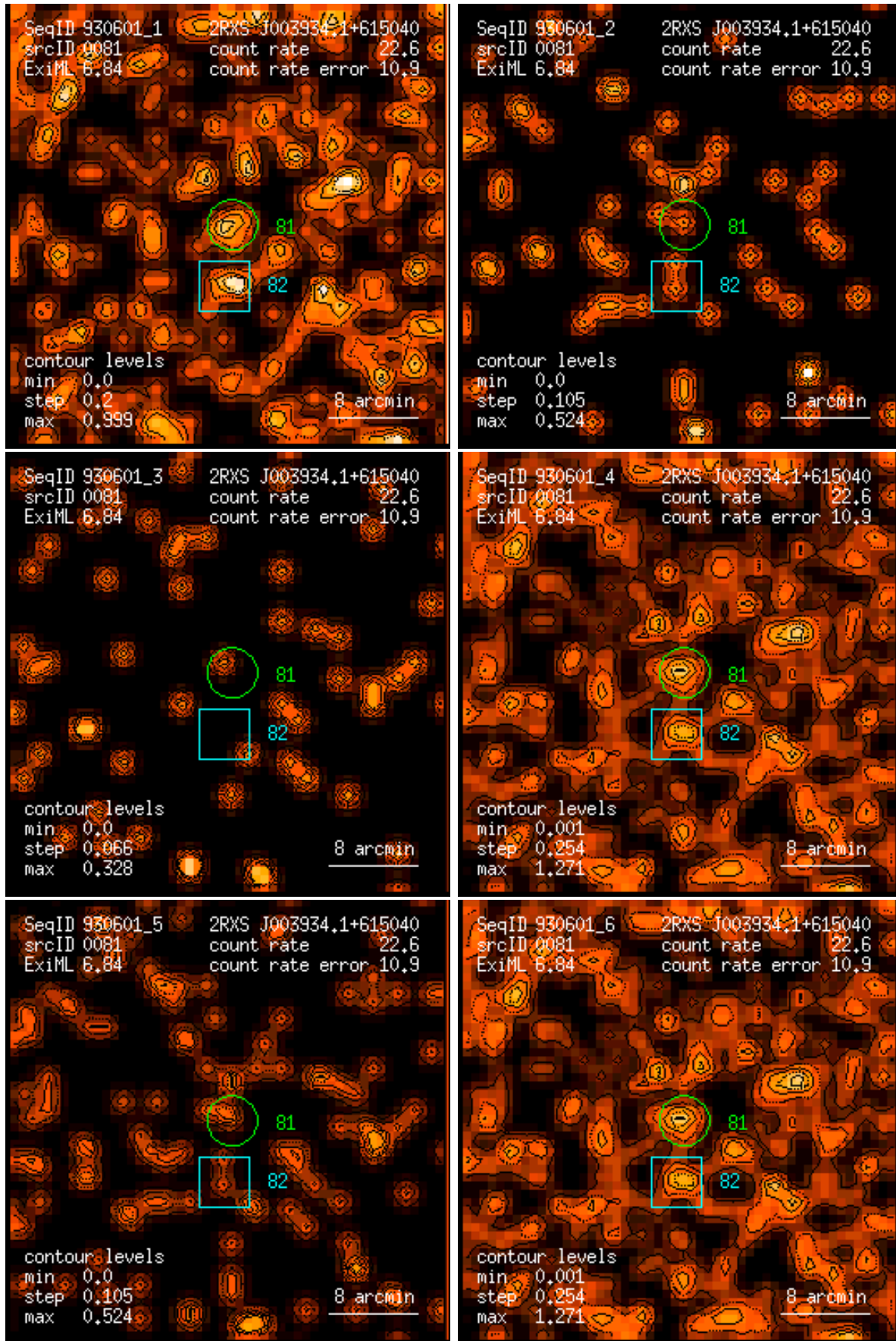
Figure 81: RASS 930601: detection 0081: band rate images, Gaussian filter: (1) PSPC channels 11 – 41, (2) 52 – 90, (3) 91 – 201, (4) 11 – 235, (5) 52 – 201, (6) 11 – 201. Broad band rates in counts/ks. Band rate contour levels in counts/ks/arcmin 2 .
