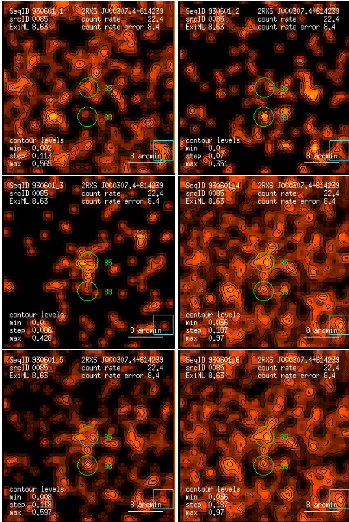
Figure 85: RASS 930601: detection 0085: band rate images, Gaussian filter: (1) PSPC channels 11 – 41, (2) 52 – 90, (3) 91 – 201, (4) 11 – 235, (5) 52 – 201, (6) 11 – 201. Broad band rates in counts/ks. Band rate contour levels in counts/ks/arcmin 2 .
