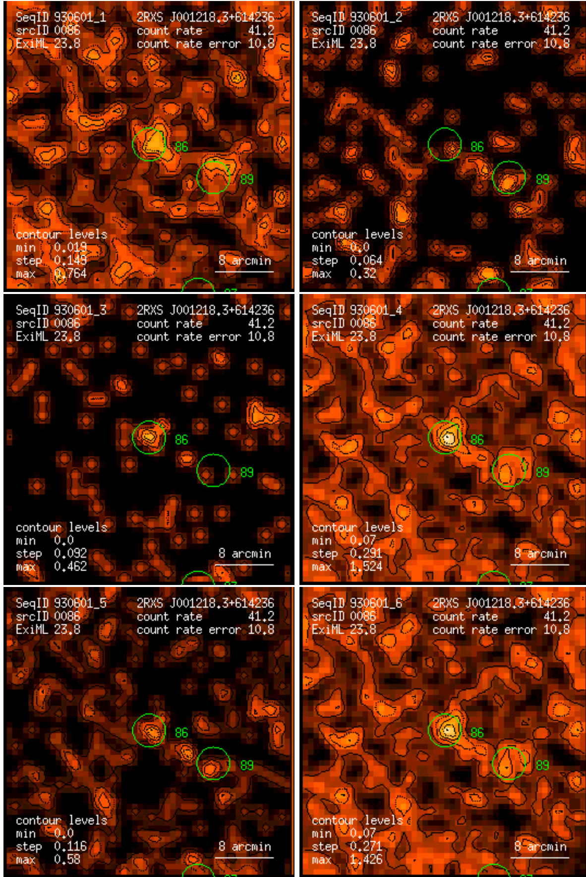
Figure 86: RASS 930601: detection 0086: band rate images, Gaussian filter: (1) PSPC channels 11 – 41, (2) 52 – 90, (3) 91 – 201, (4) 11 – 235, (5) 52 – 201, (6) 11 – 201. Broad band rates in counts/ks. Band rate contour levels in counts/ks/arcmin 2 .
