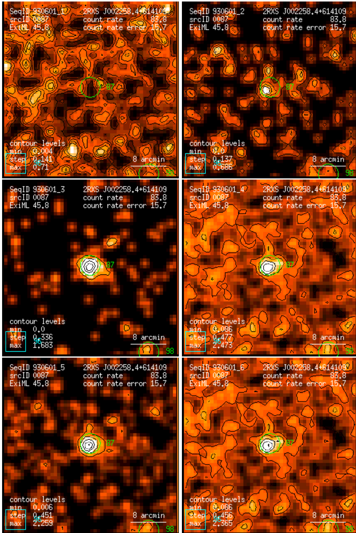
Figure 87: RASS 930601: detection 0087: band rate images, Gaussian filter: (1) PSPC channels 11 – 41, (2) 52 – 90, (3) 91 – 201, (4) 11 – 235, (5) 52 – 201, (6) 11 – 201. Broad band rates in counts/ks. Band rate contour levels in counts/ks/arcmin 2 .
