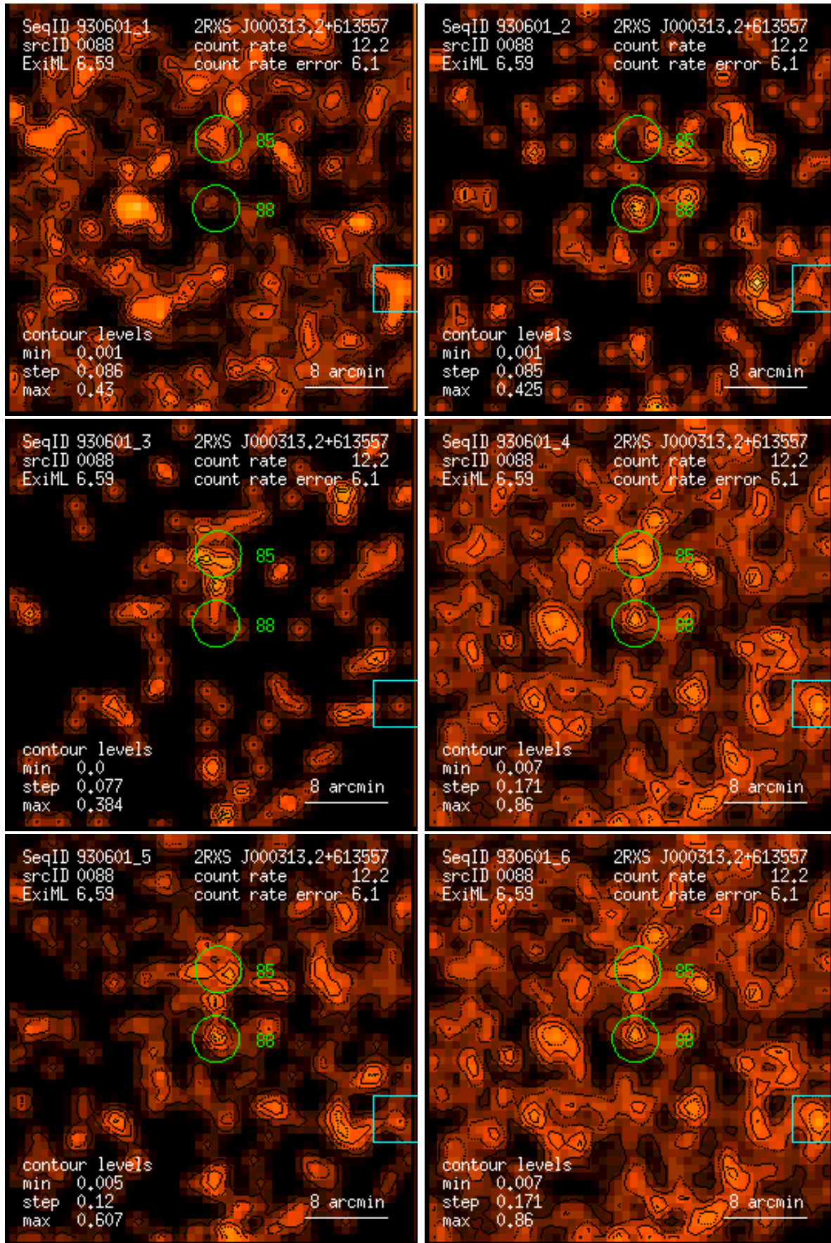
Figure 88: RASS 930601: detection 0088: band rate images, Gaussian filter: (1) PSPC channels 11 – 41, (2) 52 – 90, (3) 91 – 201, (4) 11 – 235, (5) 52 – 201, (6) 11 – 201. Broad band rates in counts/ks. Band rate contour levels in counts/ks/arcmin 2 .
