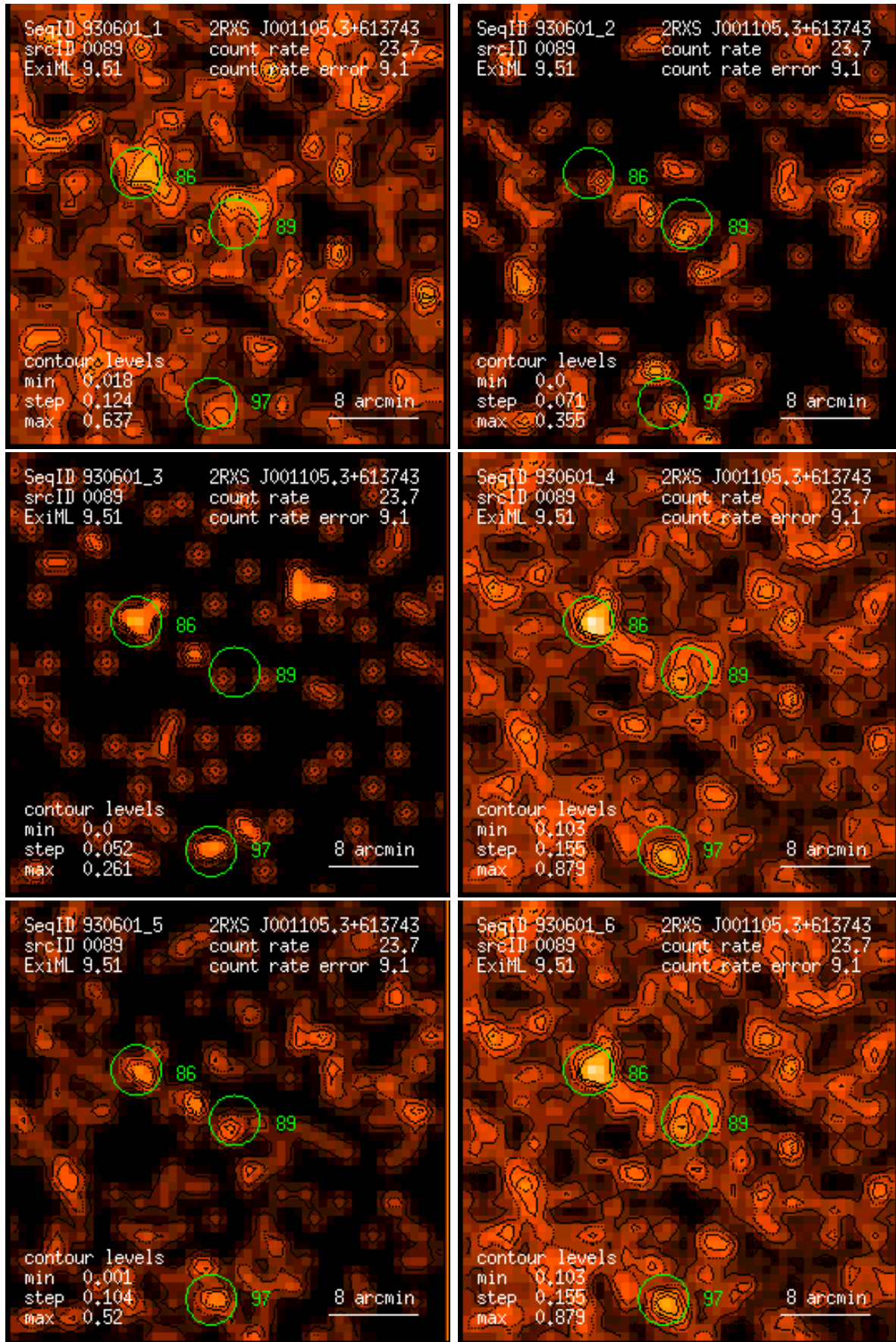
Figure 89: RASS 930601: detection 0089: band rate images, Gaussian filter: (1) PSPC channels 11 – 41, (2) 52 – 90, (3) 91 – 201, (4) 11 – 235, (5) 52 – 201, (6) 11 – 201. Broad band rates in counts/ks. Band rate contour levels in counts/ks/arcmin 2 .
