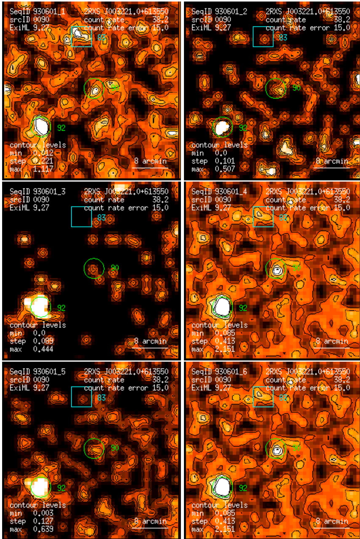
Figure 90: RASS 930601: detection 0090: band rate images, Gaussian filter: (1) PSPC channels 11 – 41, (2) 52 – 90, (3) 91 – 201, (4) 11 – 235, (5) 52 – 201, (6) 11 – 201. Broad band rates in counts/ks. Band rate contour levels in counts/ks/arcmin 2 .
