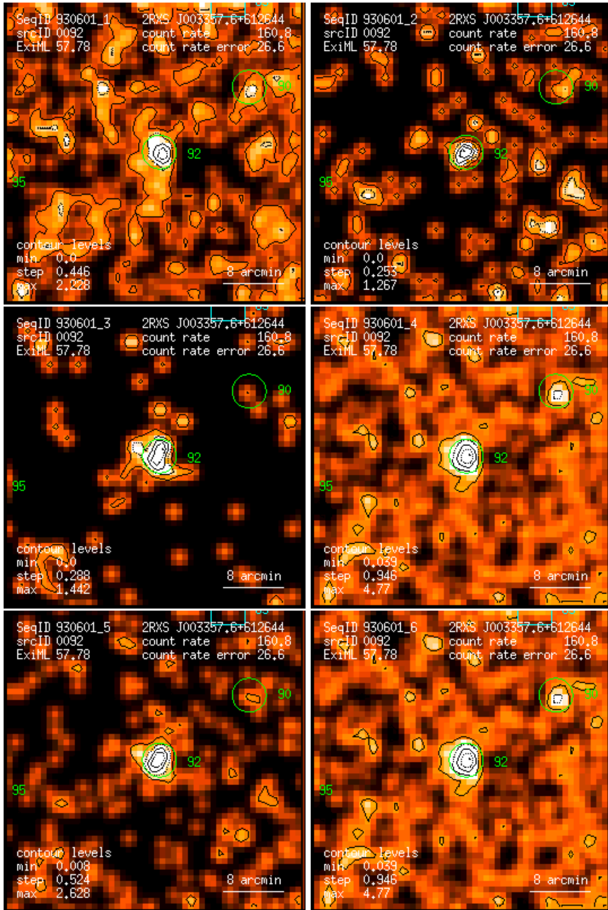
Figure 92: RASS 930601: detection 0092: band rate images, Gaussian filter: (1) PSPC channels 11 – 41, (2) 52 – 90, (3) 91 – 201, (4) 11 – 235, (5) 52 – 201, (6) 11 – 201. Broad band rates in counts/ks. Band rate contour levels in counts/ks/arcmin 2 .
