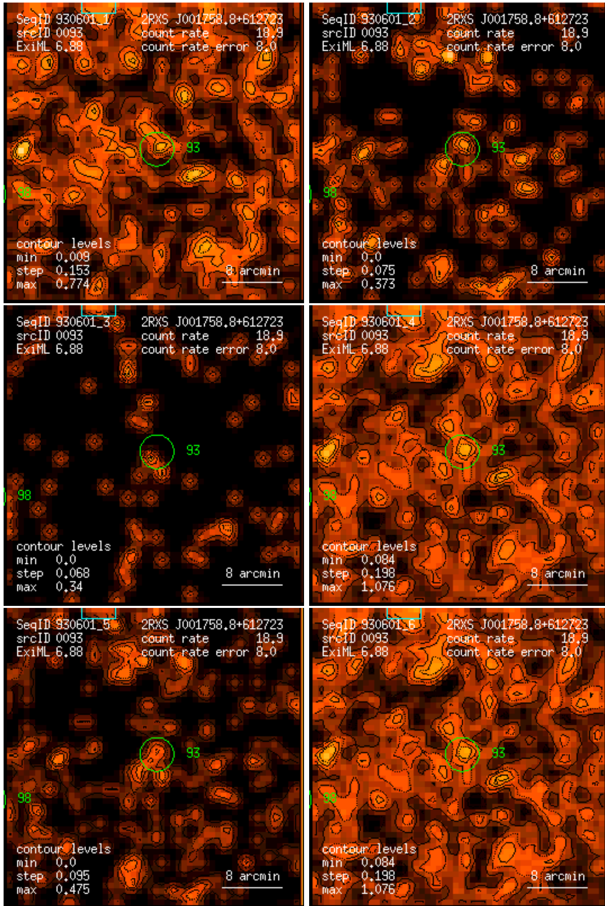
Figure 93: RASS 930601: detection 0093: band rate images, Gaussian filter: (1) PSPC channels 11 – 41, (2) 52 – 90, (3) 91 – 201, (4) 11 – 235, (5) 52 – 201, (6) 11 – 201. Broad band rates in counts/ks. Band rate contour levels in counts/ks/arcmin 2 .
