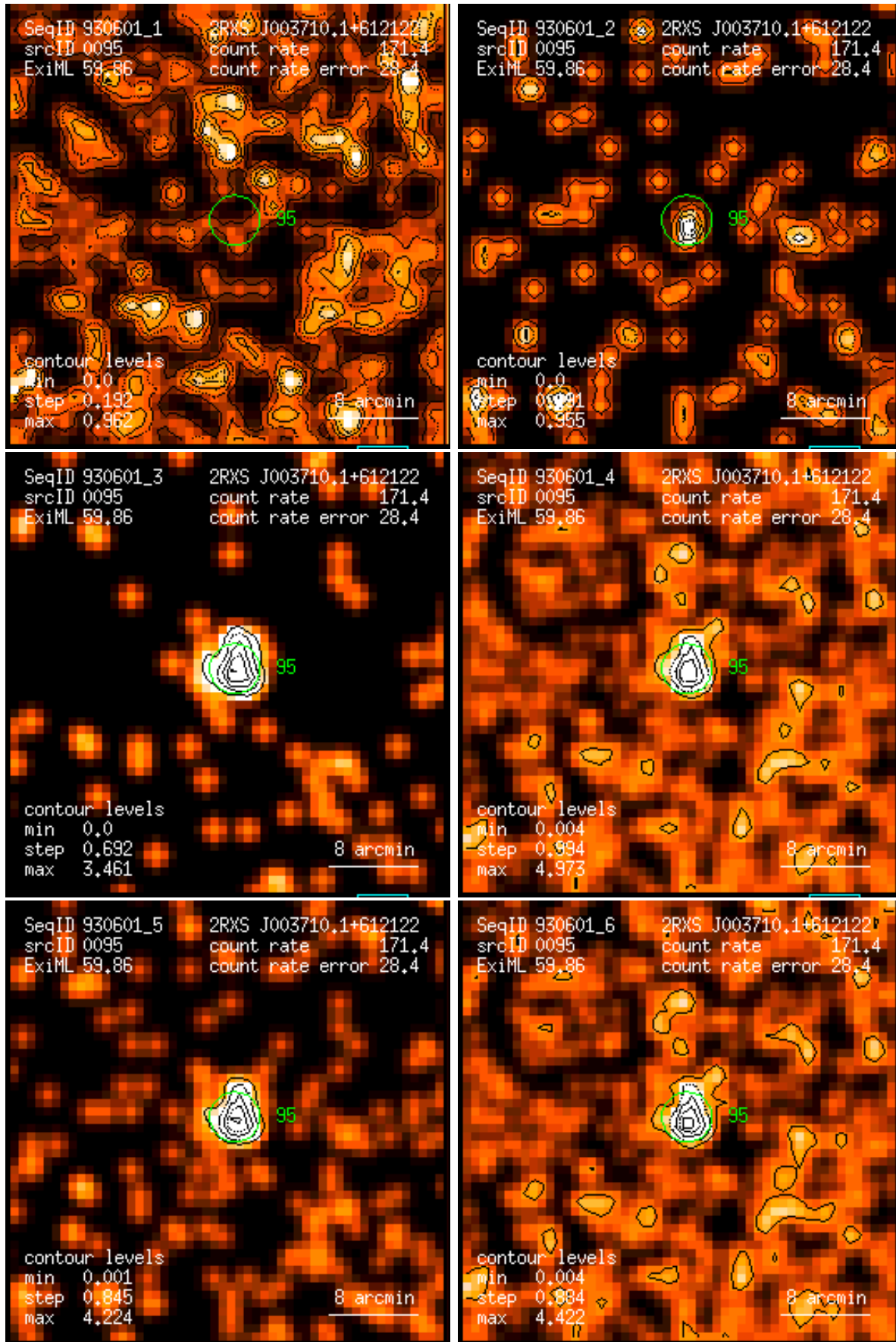
Figure 95: RASS 930601: detection 0095: band rate images, Gaussian filter: (1) PSPC channels 11 – 41, (2) 52 – 90, (3) 91 – 201, (4) 11 – 235, (5) 52 – 201, (6) 11 – 201. Broad band rates in counts/ks. Band rate contour levels in counts/ks/arcmin 2 .
