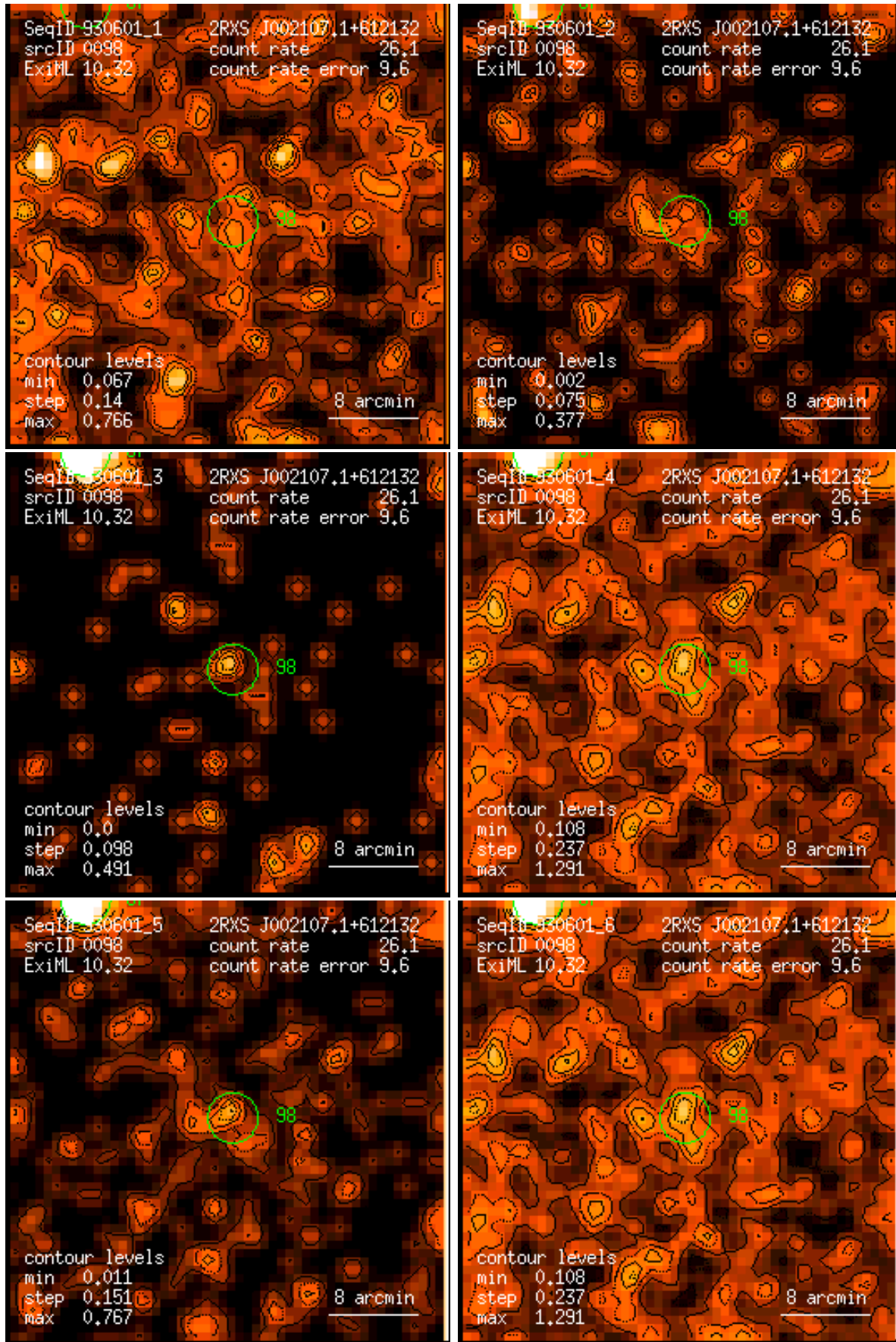
Figure 98: RASS 930601: detection 0098: band rate images, Gaussian filter: (1) PSPC channels 11 – 41, (2) 52 – 90, (3) 91 – 201, (4) 11 – 235, (5) 52 – 201, (6) 11 – 201. Broad band rates in counts/ks. Band rate contour levels in counts/ks/arcmin 2 .
