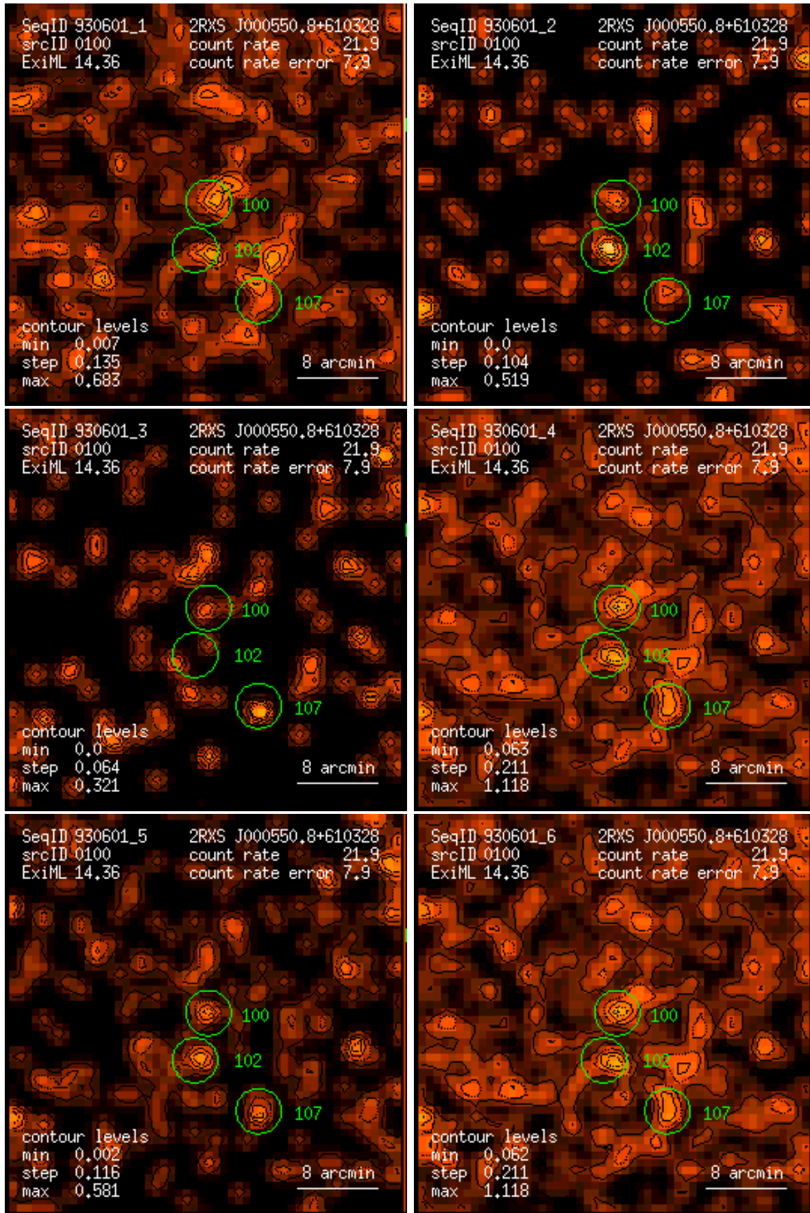
Figure 100: RASS 930601: detection 0100: band rate images, Gaussian filter: (1) PSPC channels 11 – 41, (2) 52 – 90, (3) 91 – 201, (4) 11 – 235, (5) 52 – 201, (6) 11 – 201. Broad band rates in counts/ks. Band rate contour levels in counts/ks/arcmin 2 .
