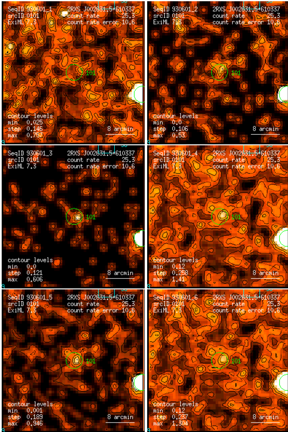
Figure 101: RASS 930601: detection 0101: band rate images, Gaussian filter: (1) PSPC channels 11 – 41, (2) 52 – 90, (3) 91 – 201, (4) 11 – 235, (5) 52 – 201, (6) 11 – 201. Broad band rates in counts/ks. Band rate contour levels in counts/ks/arcmin 2 .
