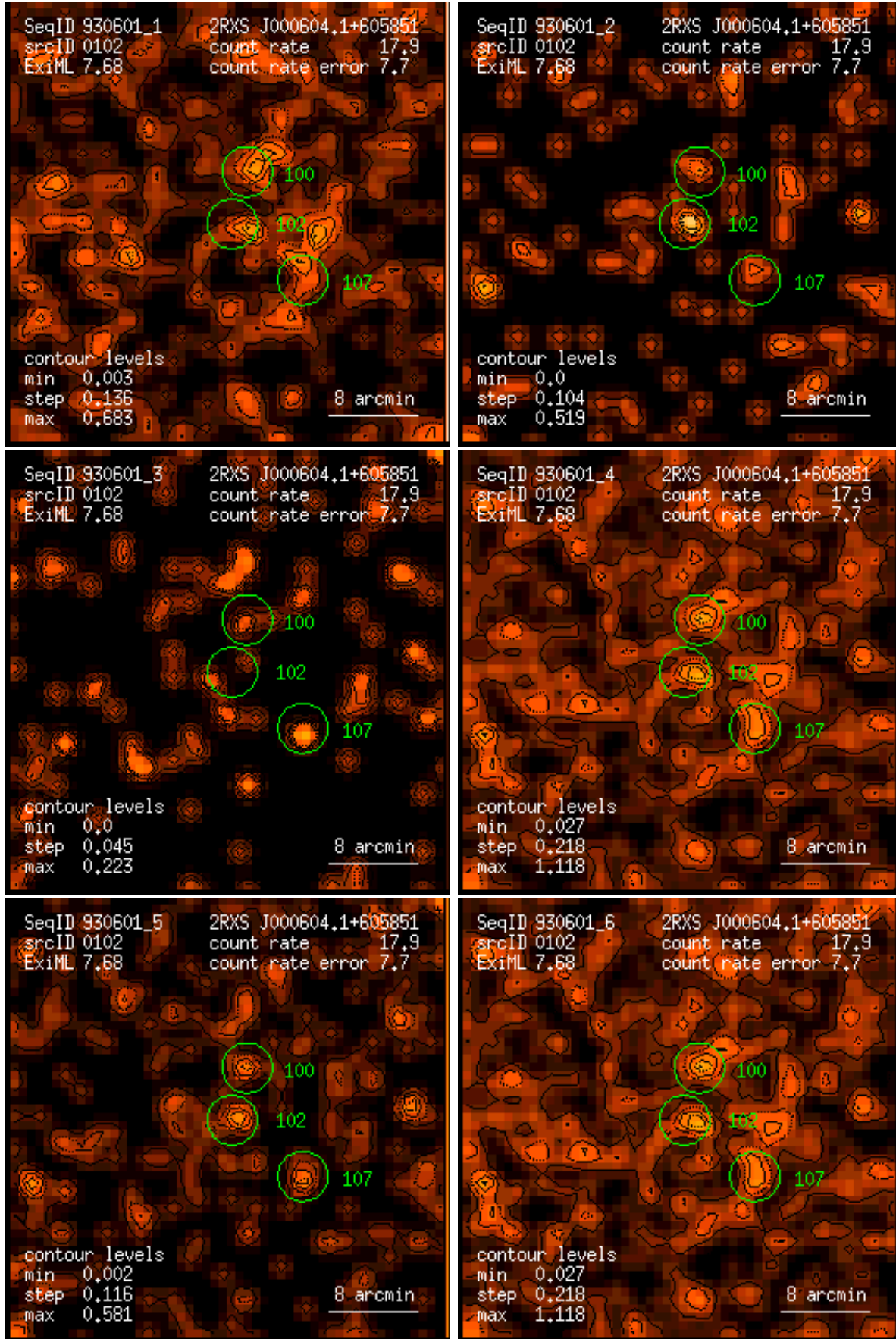
Figure 102: RASS 930601: detection 0102: band rate images, Gaussian filter: (1) PSPC channels 11 – 41, (2) 52 – 90, (3) 91 – 201, (4) 11 – 235, (5) 52 – 201, (6) 11 – 201. Broad band rates in counts/ks. Band rate contour levels in counts/ks/arcmin 2 .
