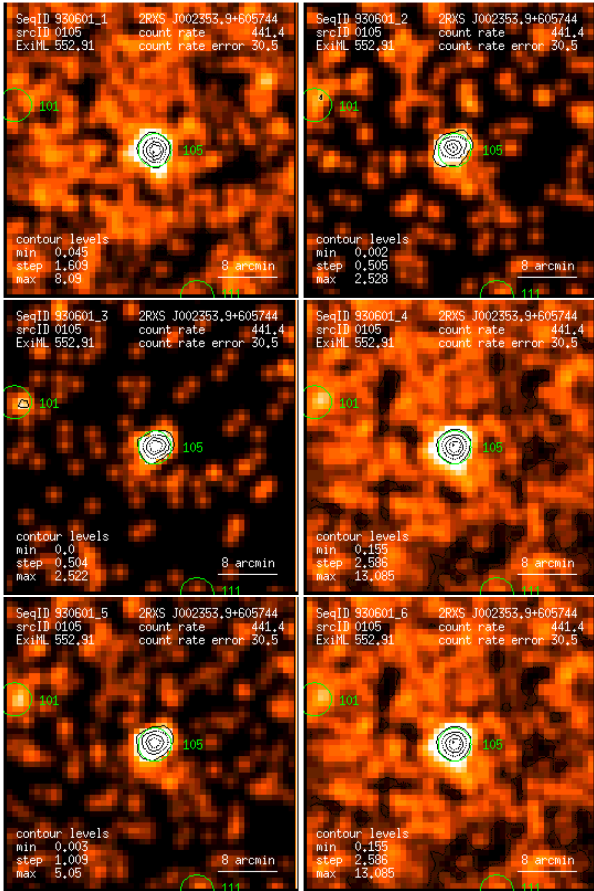
Figure 105: RASS 930601: detection 0105: band rate images, Gaussian filter: (1) PSPC channels 11 – 41, (2) 52 – 90, (3) 91 – 201, (4) 11 – 235, (5) 52 – 201, (6) 11 – 201. Broad band rates in counts/ks. Band rate contour levels in counts/ks/arcmin 2 .
