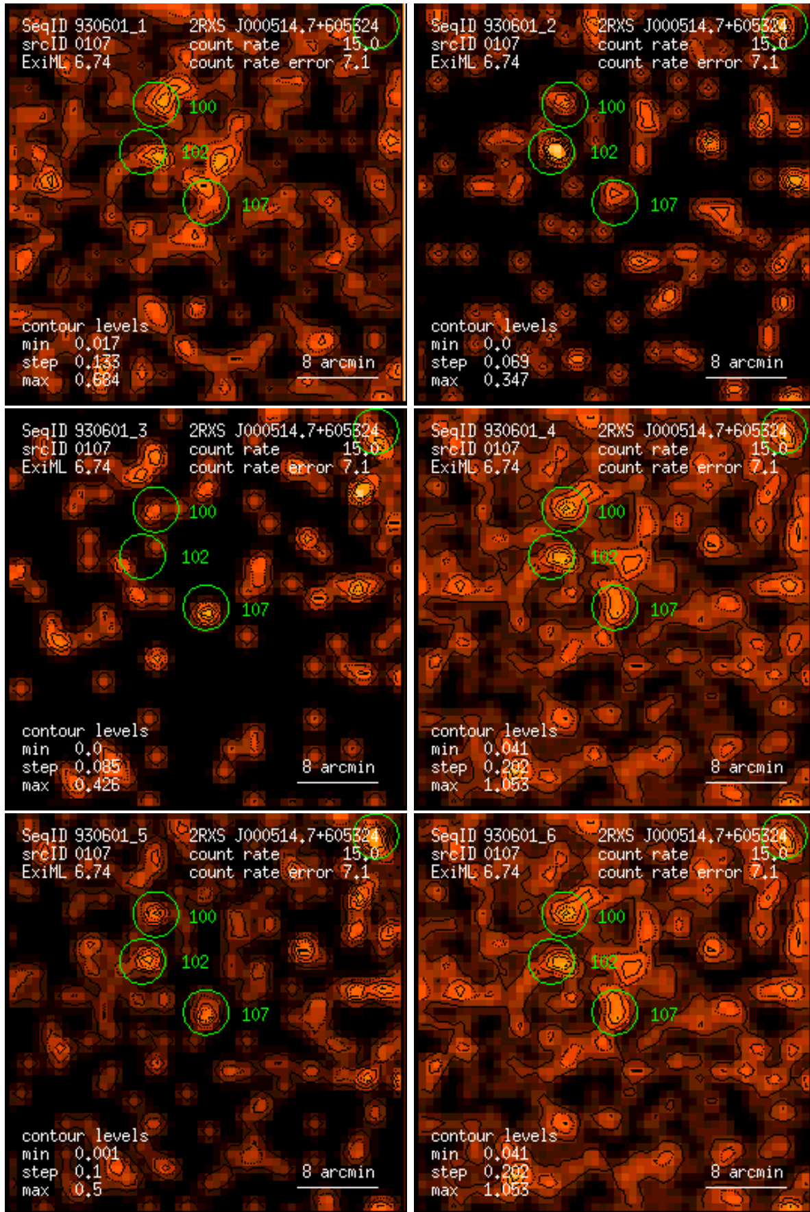
Figure 107: RASS 930601: detection 0107: band rate images, Gaussian filter: (1) PSPC channels 11 – 41, (2) 52 – 90, (3) 91 – 201, (4) 11 – 235, (5) 52 – 201, (6) 11 – 201. Broad band rates in counts/ks. Band rate contour levels in counts/ks/arcmin 2 .
