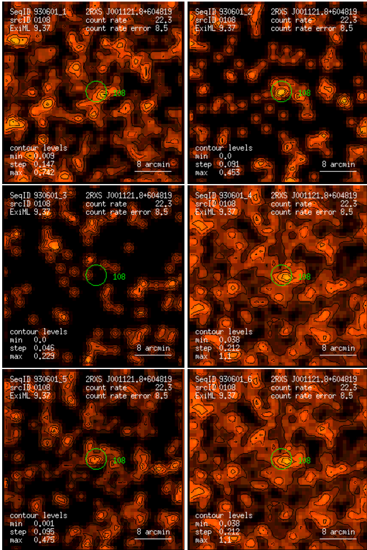
Figure 108: RASS 930601: detection 0108: band rate images, Gaussian filter: (1) PSPC channels 11 – 41, (2) 52 – 90, (3) 91 – 201, (4) 11 – 235, (5) 52 – 201, (6) 11 – 201. Broad band rates in counts/ks. Band rate contour levels in counts/ks/arcmin 2 .
