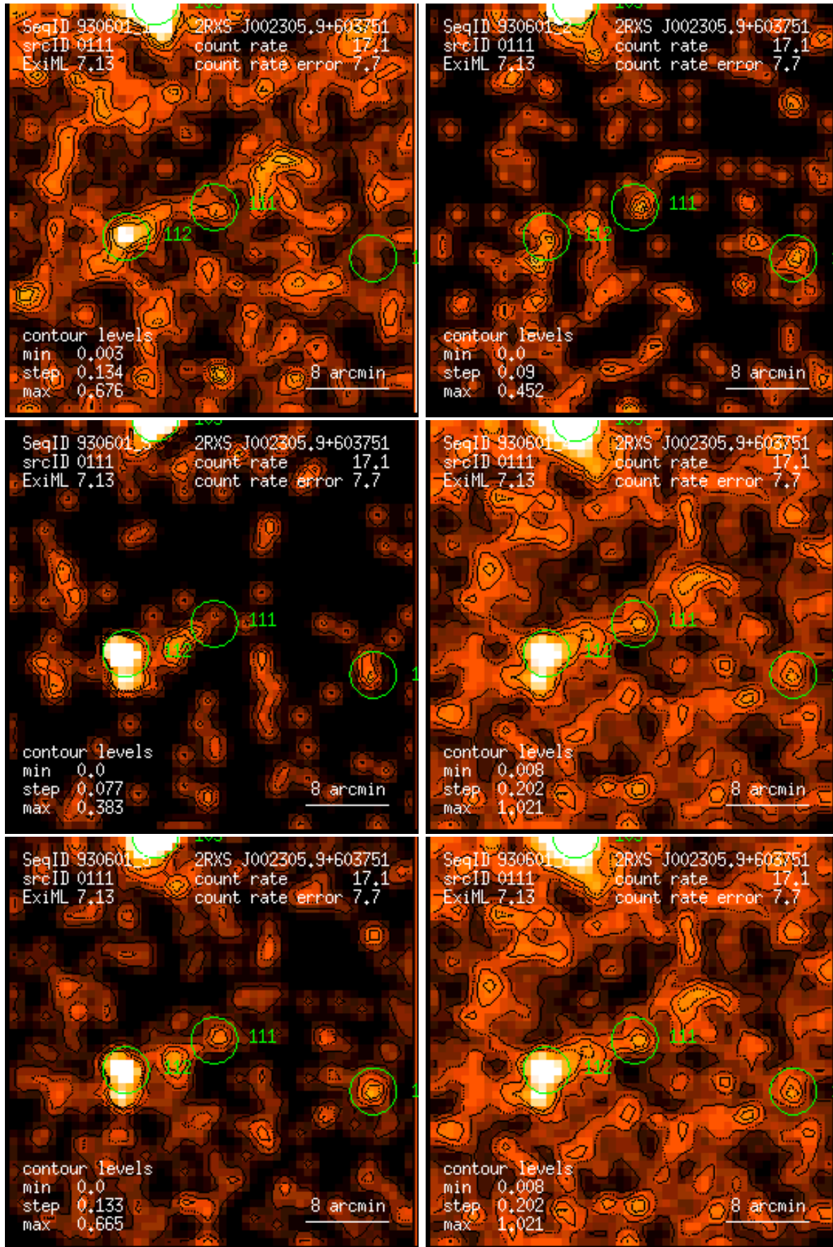
Figure 111: RASS 930601: detection 0111: band rate images, Gaussian filter: (1) PSPC channels 11 – 41, (2) 52 – 90, (3) 91 – 201, (4) 11 – 235, (5) 52 – 201, (6) 11 – 201. Broad band rates in counts/ks. Band rate contour levels in counts/ks/arcmin 2 .
