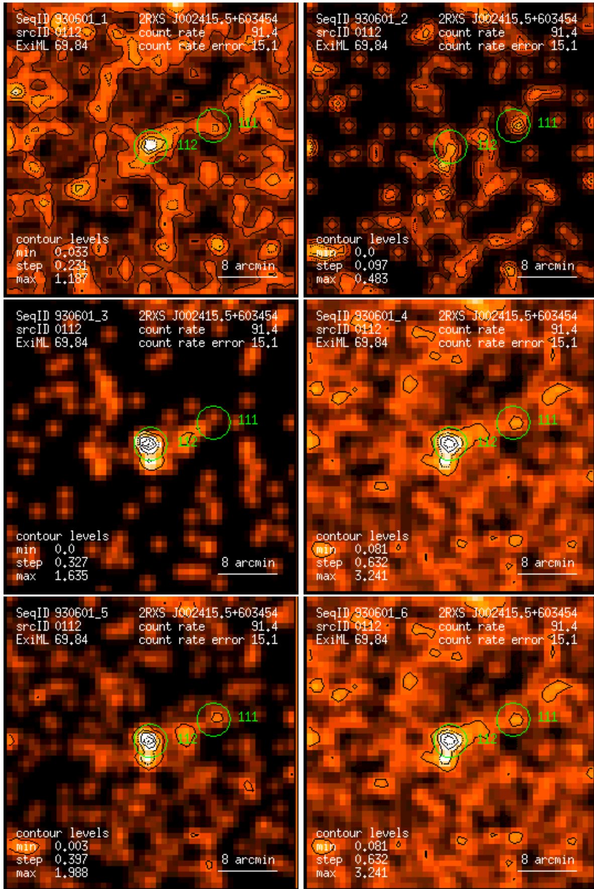
Figure 112: RASS 930601: detection 0112: band rate images, Gaussian filter: (1) PSPC channels 11 – 41, (2) 52 – 90, (3) 91 – 201, (4) 11 – 235, (5) 52 – 201, (6) 11 – 201. Broad band rates in counts/ks. Band rate contour levels in counts/ks/arcmin 2 .
