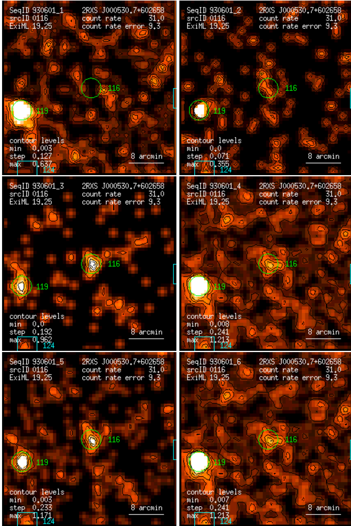
Figure 116: RASS 930601: detection 0116: band rate images, Gaussian filter: (1) PSPC channels 11 – 41, (2) 52 – 90, (3) 91 – 201, (4) 11 – 235, (5) 52 – 201, (6) 11 – 201. Broad band rates in counts/ks. Band rate contour levels in counts/ks/arcmin 2 .
