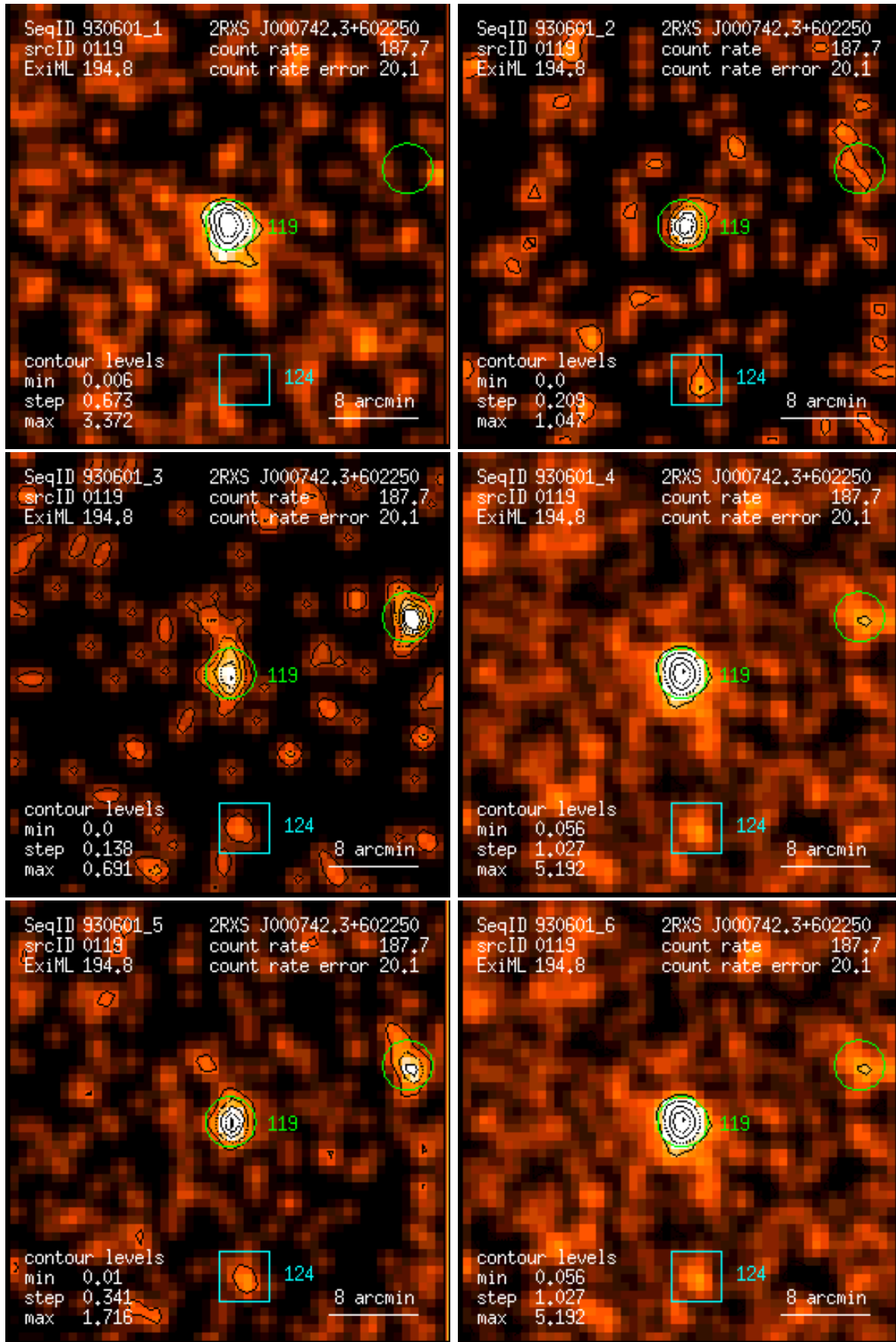
Figure 119: RASS 930601: detection 0119: band rate images, Gaussian filter: (1) PSPC channels 11 – 41, (2) 52 – 90, (3) 91 – 201, (4) 11 – 235, (5) 52 – 201, (6) 11 – 201. Broad band rates in counts/ks. Band rate contour levels in counts/ks/arcmin 2 .
