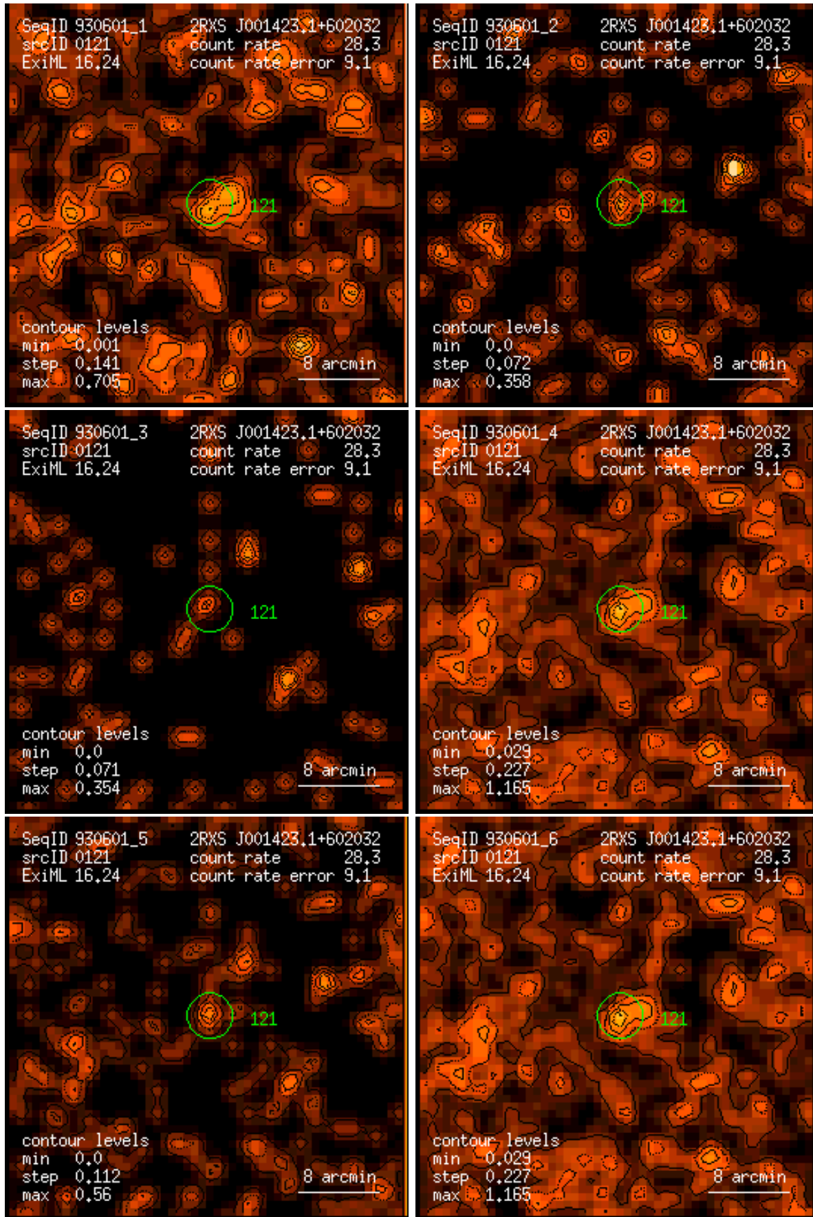
Figure 121: RASS 930601: detection 0121: band rate images, Gaussian filter: (1) PSPC channels 11 – 41, (2) 52 – 90, (3) 91 – 201, (4) 11 – 235, (5) 52 – 201, (6) 11 – 201. Broad band rates in counts/ks. Band rate contour levels in counts/ks/arcmin 2 .
