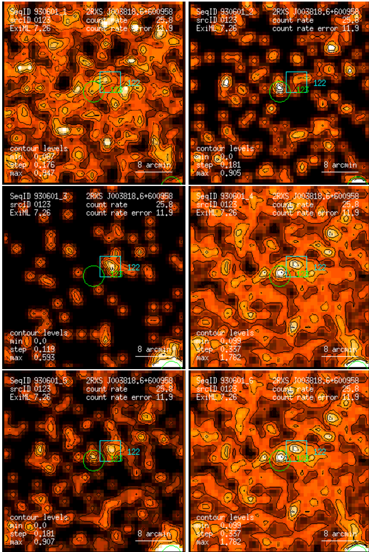
Figure 123: RASS 930601: detection 0123: band rate images, Gaussian filter: (1) PSPC channels 11 – 41, (2) 52 – 90, (3) 91 – 201, (4) 11 – 235, (5) 52 – 201, (6) 11 – 201. Broad band rates in counts/ks. Band rate contour levels in counts/ks/arcmin 2 .
