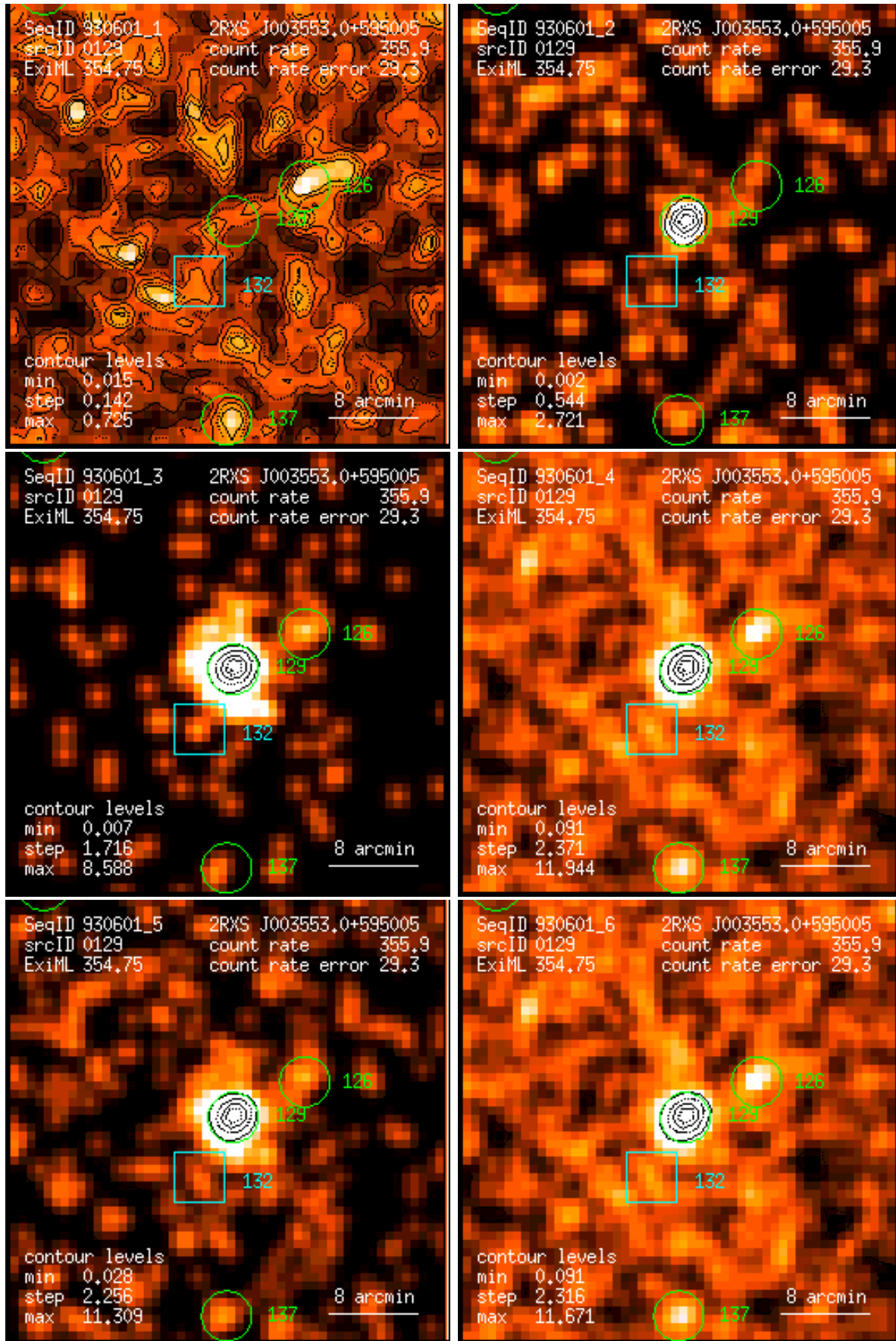
Figure 129: RASS 930601: detection 0129: band rate images, Gaussian filter: (1) PSPC channels 11 – 41, (2) 52 – 90, (3) 91 – 201, (4) 11 – 235, (5) 52 – 201, (6) 11 – 201. Broad band rates in counts/ks. Band rate contour levels in counts/ks/arcmin 2 .
