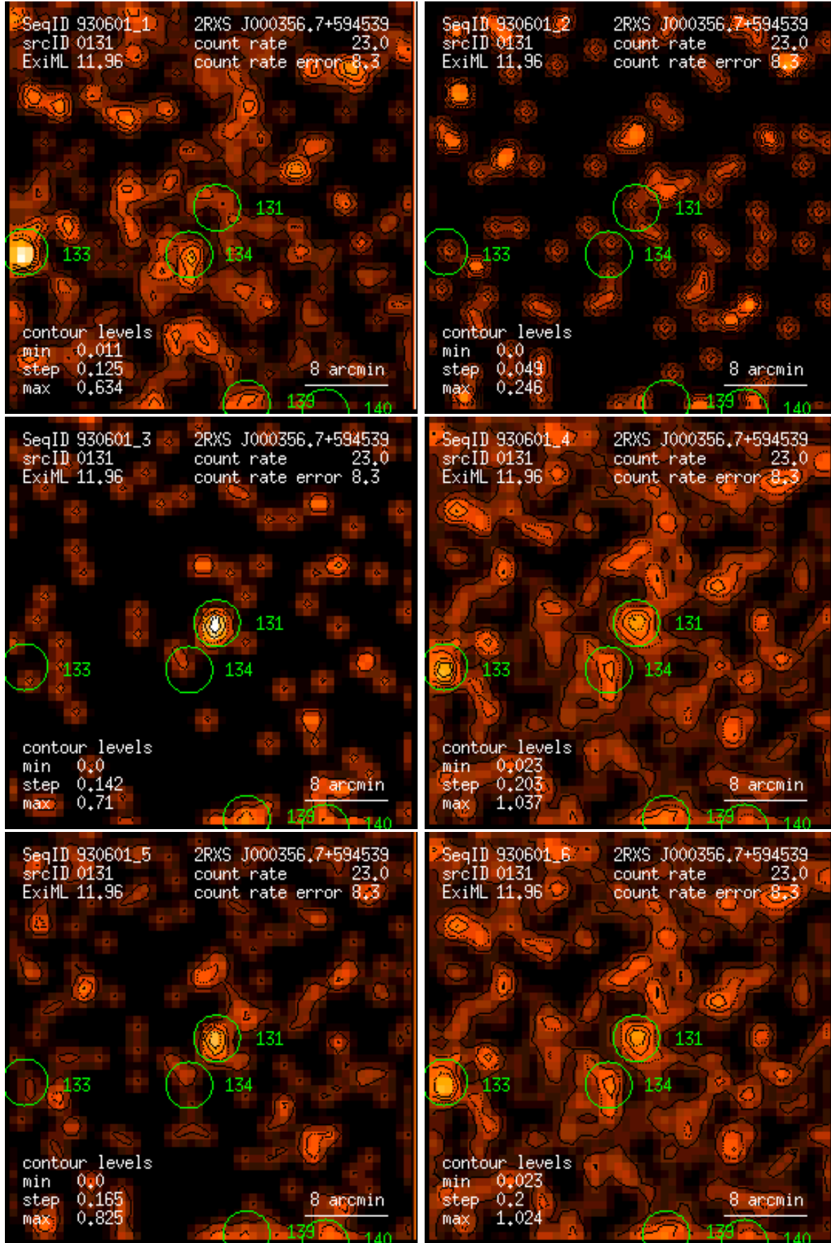
Figure 131: RASS 930601: detection 0131: band rate images, Gaussian filter: (1) PSPC channels 11 – 41, (2) 52 – 90, (3) 91 – 201, (4) 11 – 235, (5) 52 – 201, (6) 11 – 201. Broad band rates in counts/ks. Band rate contour levels in counts/ks/arcmin 2 .
