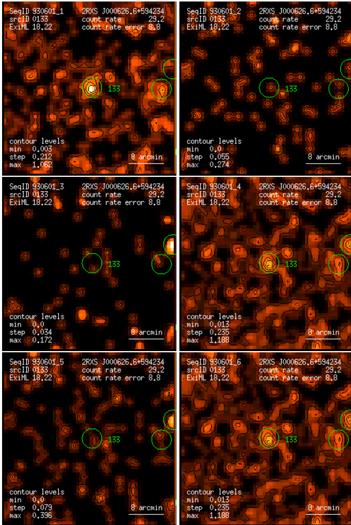
Figure 133: RASS 930601: detection 0133: band rate images, Gaussian filter: (1) PSPC channels 11 – 41, (2) 52 – 90, (3) 91 – 201, (4) 11 – 235, (5) 52 – 201, (6) 11 – 201. Broad band rates in counts/ks. Band rate contour levels in counts/ks/arcmin 2 .
