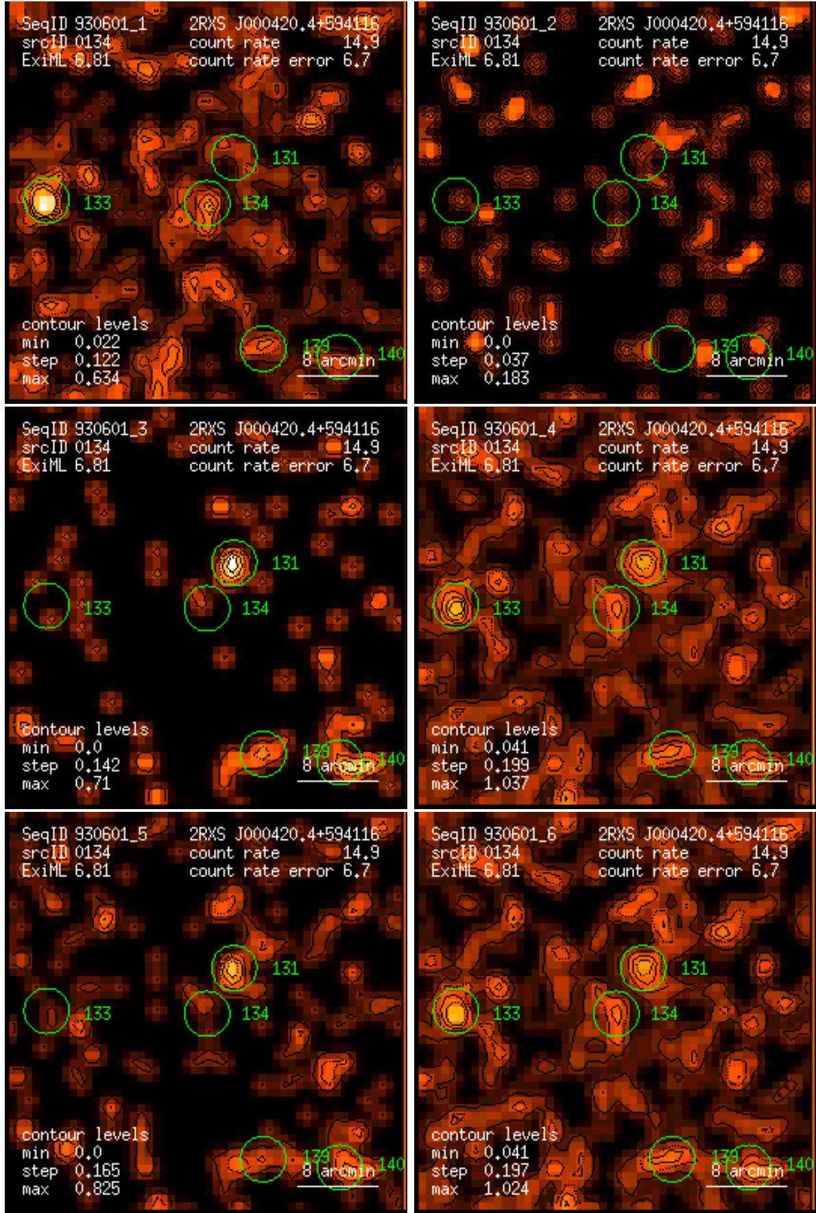
Figure 134: RASS 930601: detection 0134: band rate images, Gaussian filter: (1) PSPC channels 11 – 41, (2) 52 – 90, (3) 91 – 201, (4) 11 – 235, (5) 52 – 201, (6) 11 – 201. Broad band rates in counts/ks. Band rate contour levels in counts/ks/arcmin 2 .
