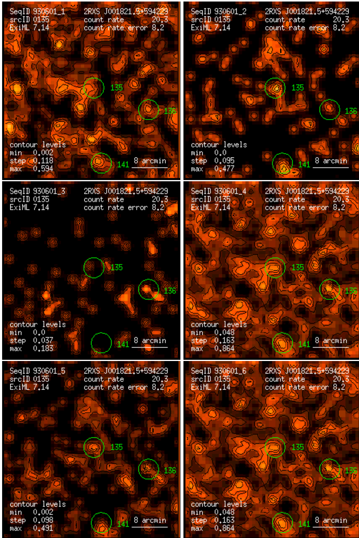
Figure 135: RASS 930601: detection 0135: band rate images, Gaussian filter: (1) PSPC channels 11 – 41, (2) 52 – 90, (3) 91 – 201, (4) 11 – 235, (5) 52 – 201, (6) 11 – 201. Broad band rates in counts/ks. Band rate contour levels in counts/ks/arcmin 2 .
