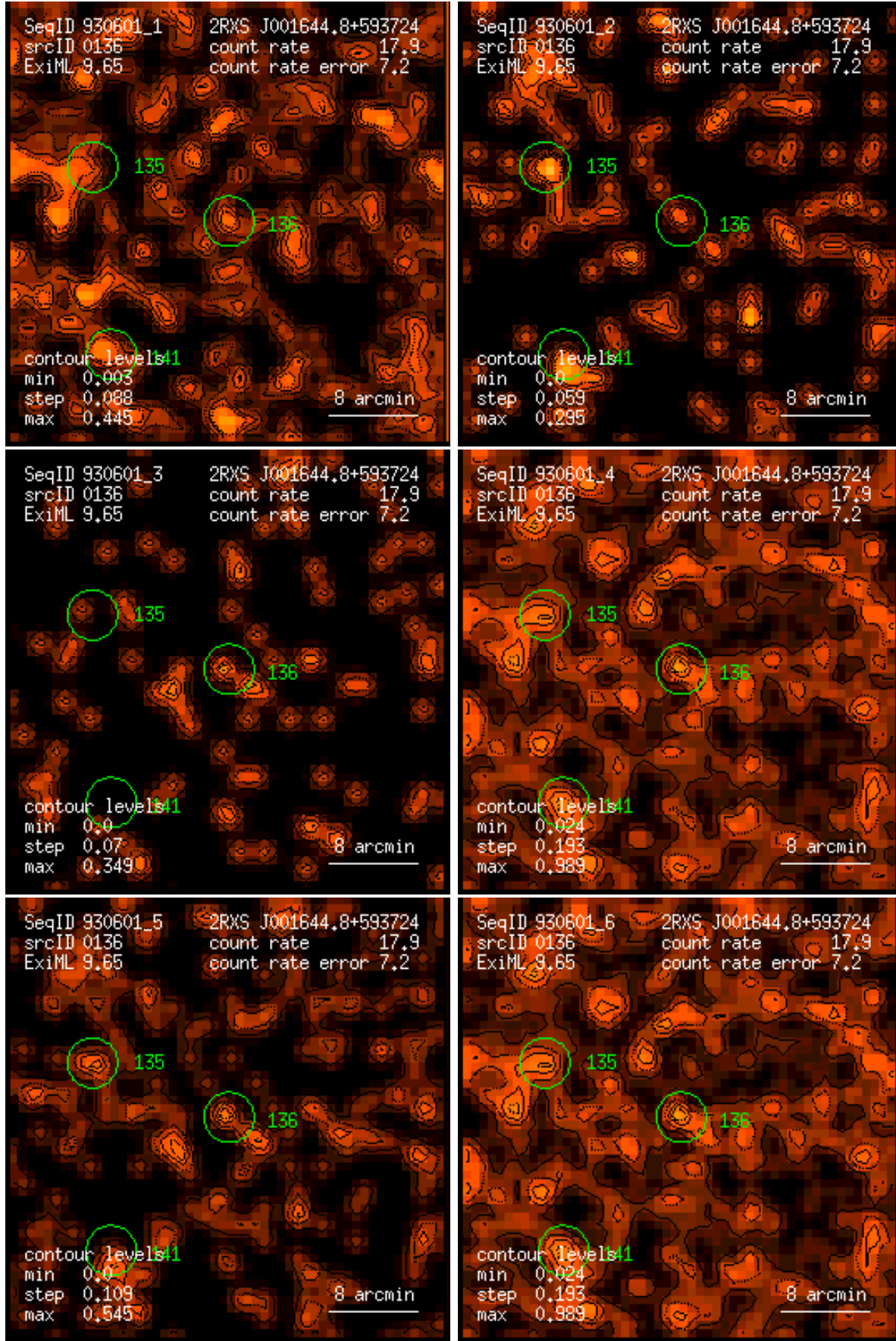
Figure 136: RASS 930601: detection 0136: band rate images, Gaussian filter: (1) PSPC channels 11 – 41, (2) 52 – 90, (3) 91 – 201, (4) 11 – 235, (5) 52 – 201, (6) 11 – 201. Broad band rates in counts/ks. Band rate contour levels in counts/ks/arcmin 2 .
