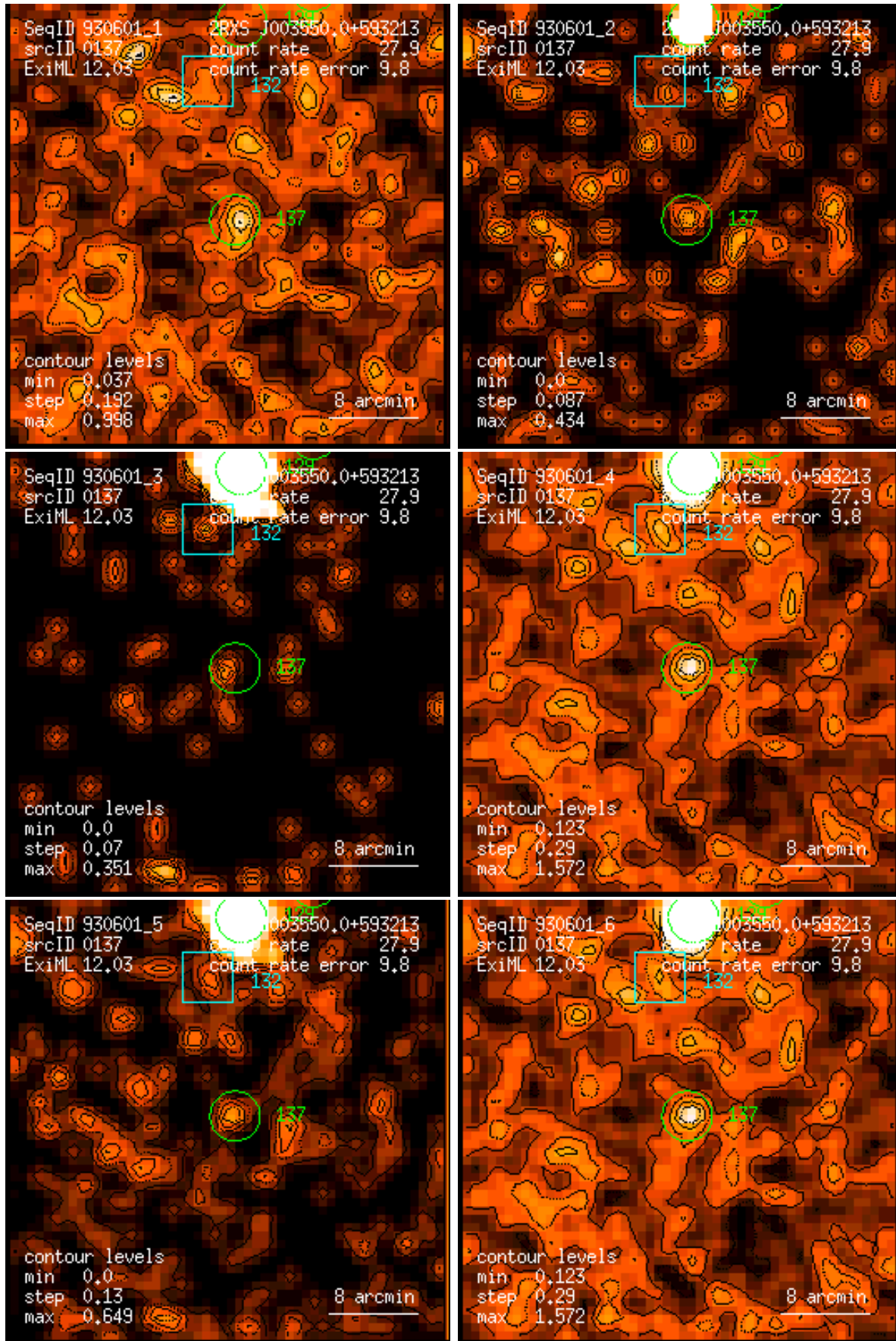
Figure 137: RASS 930601: detection 0137: band rate images, Gaussian filter: (1) PSPC channels 11 – 41, (2) 52 – 90, (3) 91 – 201, (4) 11 – 235, (5) 52 – 201, (6) 11 – 201. Broad band rates in counts/ks. Band rate contour levels in counts/ks/arcmin 2 .
