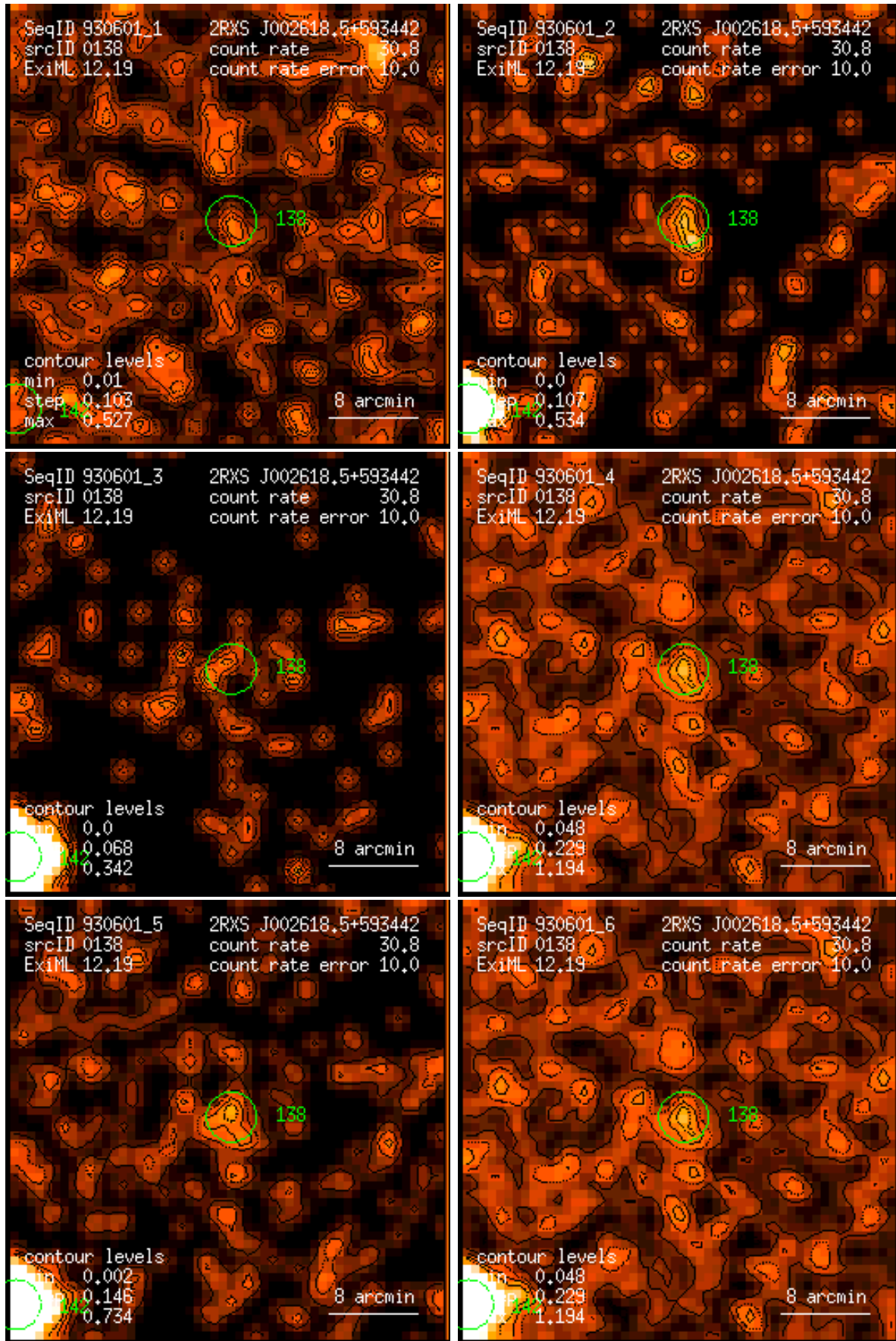
Figure 138: RASS 930601: detection 0138: band rate images, Gaussian filter: (1) PSPC channels 11 – 41, (2) 52 – 90, (3) 91 – 201, (4) 11 – 235, (5) 52 – 201, (6) 11 – 201. Broad band rates in counts/ks. Band rate contour levels in counts/ks/arcmin 2 .
