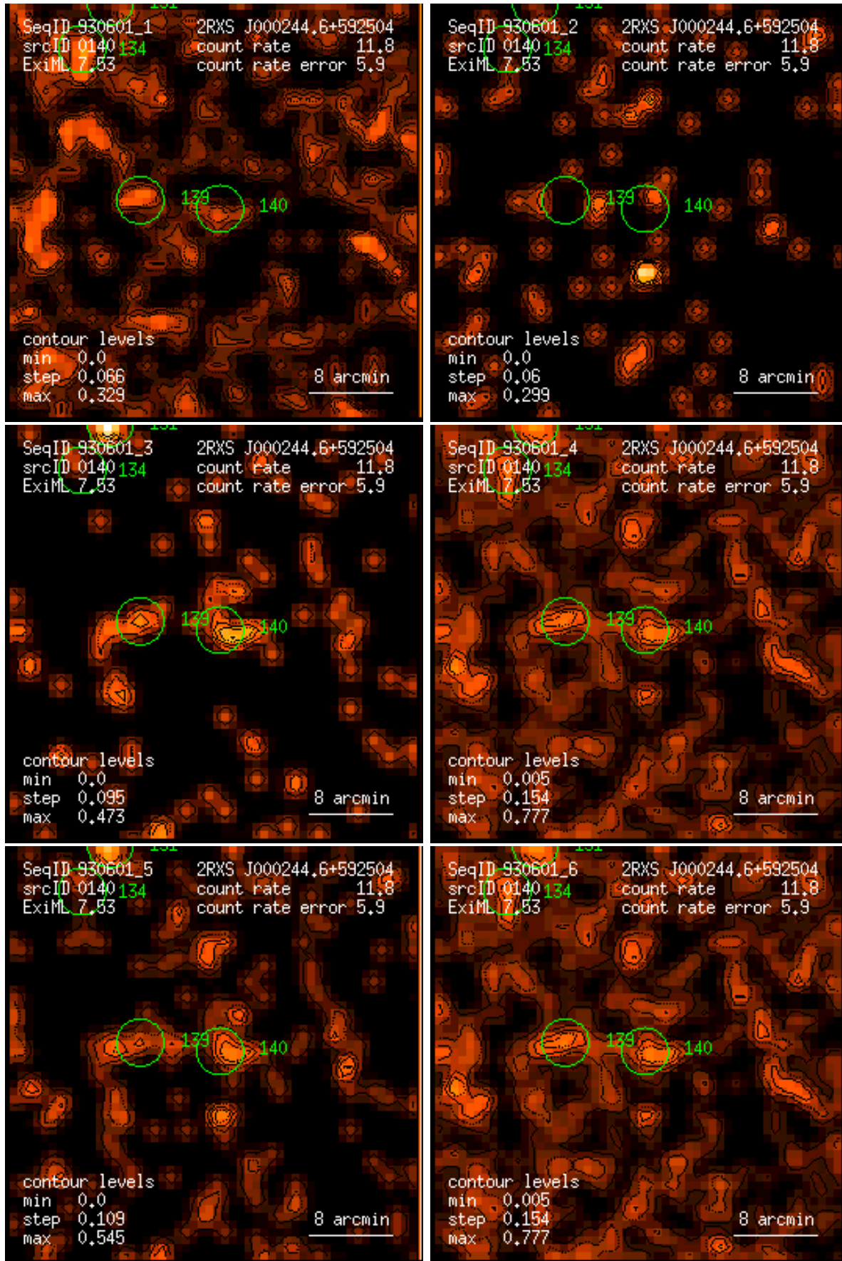
Figure 140: RASS 930601: detection 0140: band rate images, Gaussian filter: (1) PSPC channels 11 – 41, (2) 52 – 90, (3) 91 – 201, (4) 11 – 235, (5) 52 – 201, (6) 11 – 201. Broad band rates in counts/ks. Band rate contour levels in counts/ks/arcmin 2 .
