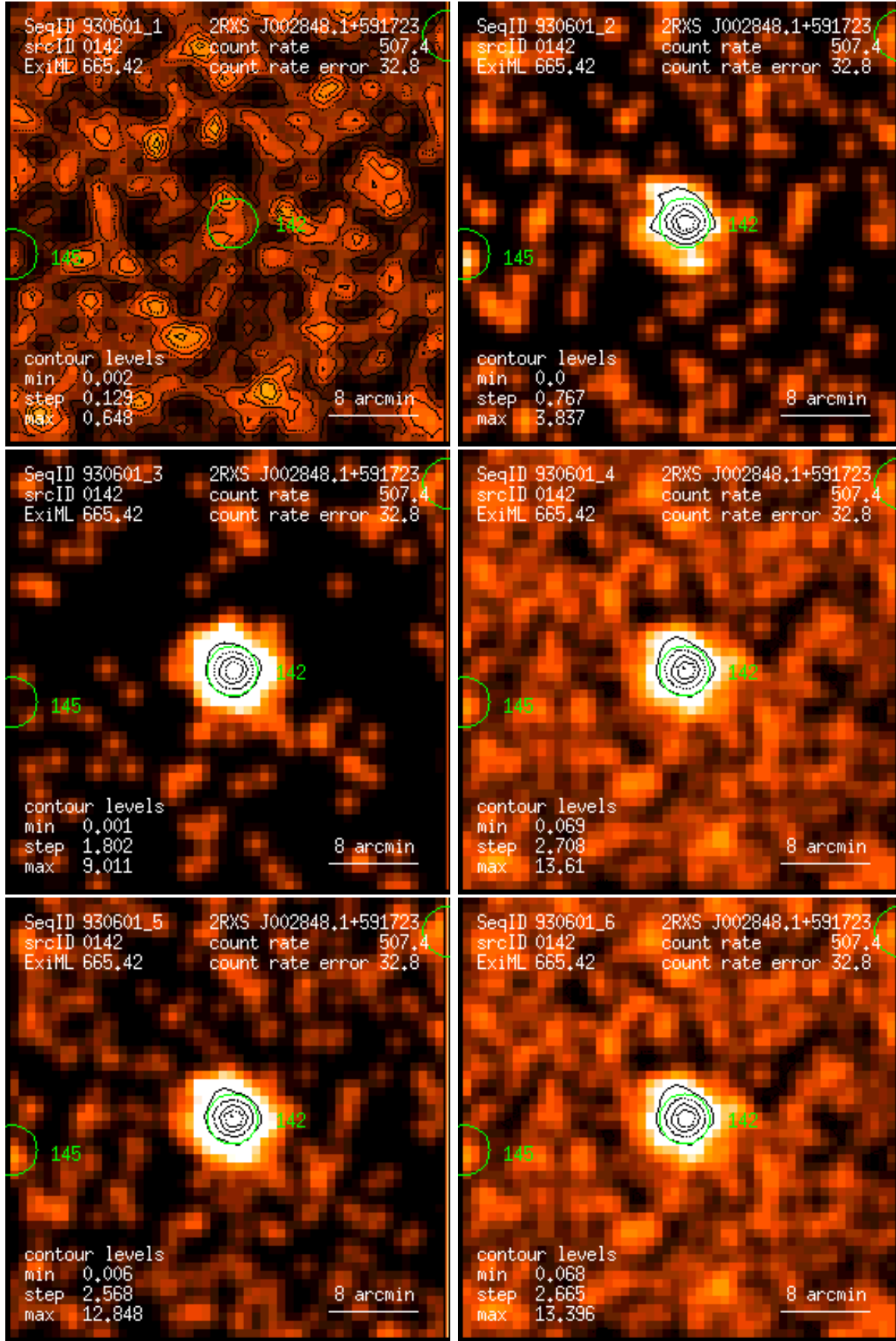
Figure 142: RASS 930601: detection 0142: band rate images, Gaussian filter: (1) PSPC channels 11 – 41, (2) 52 – 90, (3) 91 – 201, (4) 11 – 235, (5) 52 – 201, (6) 11 – 201. Broad band rates in counts/ks. Band rate contour levels in counts/ks/arcmin 2 .
