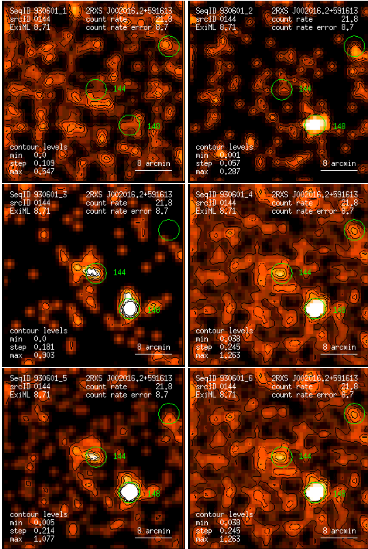
Figure 144: RASS 930601: detection 0144: band rate images, Gaussian filter: (1) PSPC channels 11 – 41, (2) 52 – 90, (3) 91 – 201, (4) 11 – 235, (5) 52 – 201, (6) 11 – 201. Broad band rates in counts/ks. Band rate contour levels in counts/ks/arcmin 2 .
