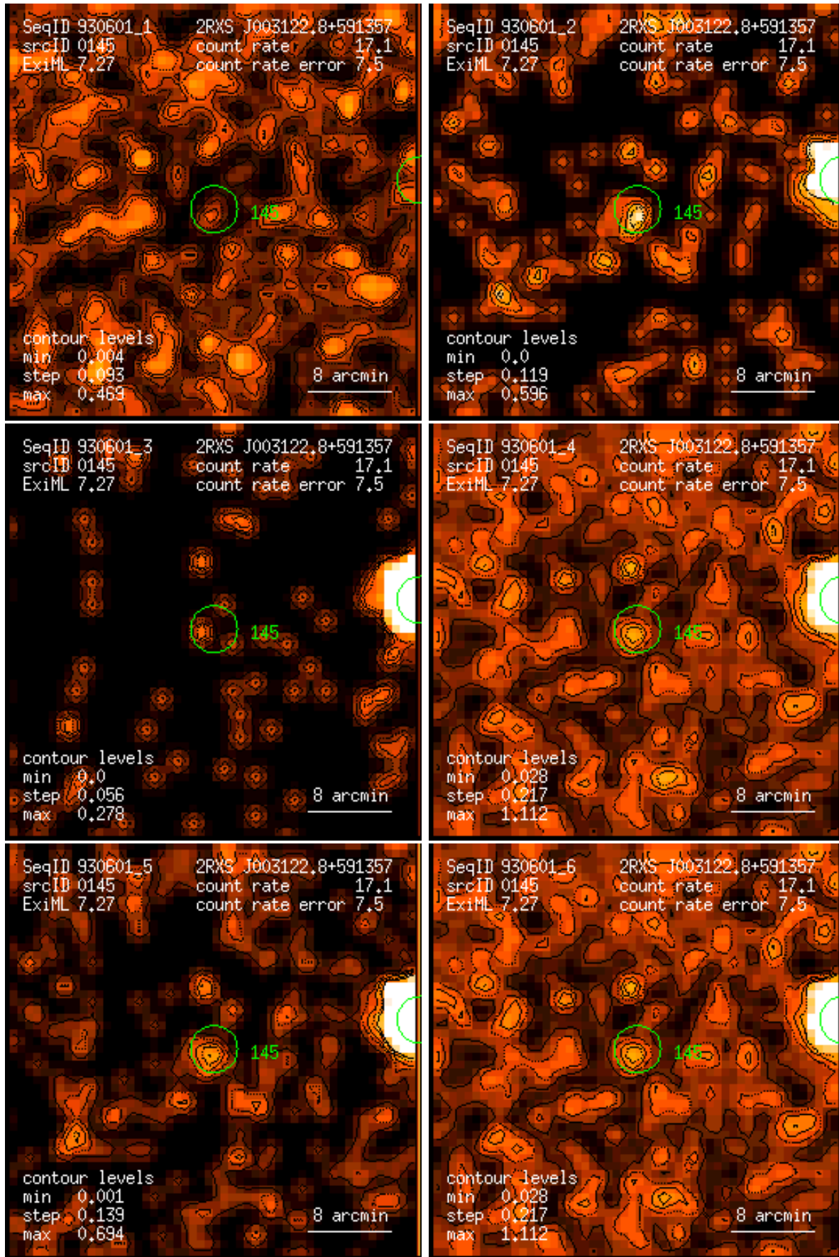
Figure 145: RASS 930601: detection 0145: band rate images, Gaussian filter: (1) PSPC channels 11 – 41, (2) 52 – 90, (3) 91 – 201, (4) 11 – 235, (5) 52 – 201, (6) 11 – 201. Broad band rates in counts/ks. Band rate contour levels in counts/ks/arcmin 2 .
