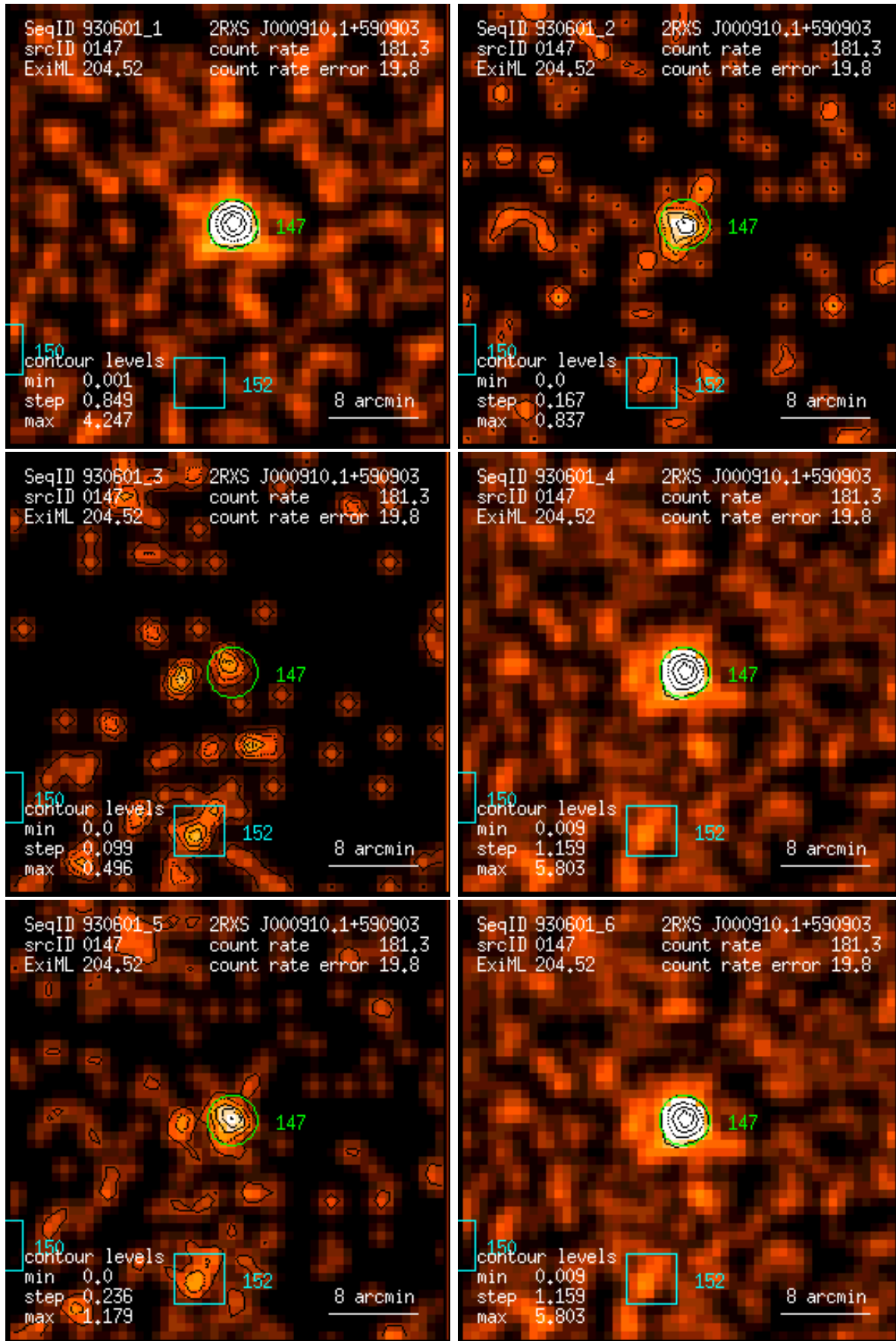
Figure 147: RASS 930601: detection 0147: band rate images, Gaussian filter: (1) PSPC channels 11 – 41, (2) 52 – 90, (3) 91 – 201, (4) 11 – 235, (5) 52 – 201, (6) 11 – 201. Broad band rates in counts/ks. Band rate contour levels in counts/ks/arcmin 2 .
